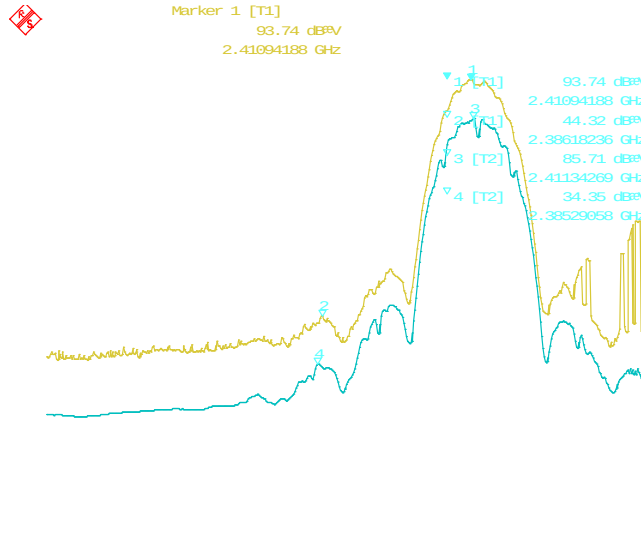
Figure 2-13: Band-Edge Compliance of RF Radiated Emission 802.11b, Channel 1, 2412 MHz, Max Pol: V, Detector: PK
