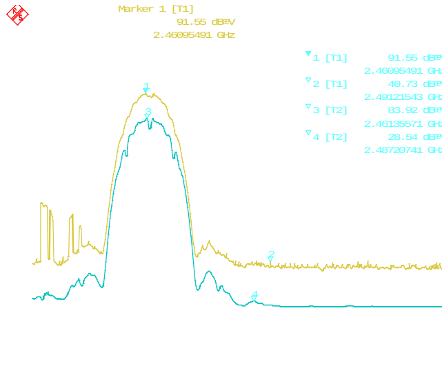
Figure 2-15: Band-Edge Compliance of RF Radiated Emission 802.11b, Channel 11, 2462 MHz, Max Pol: V, Detector: PK
