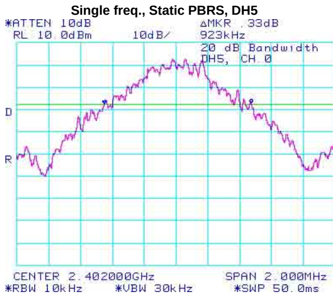
Figure 3-1: 20 dB Bandwidth
