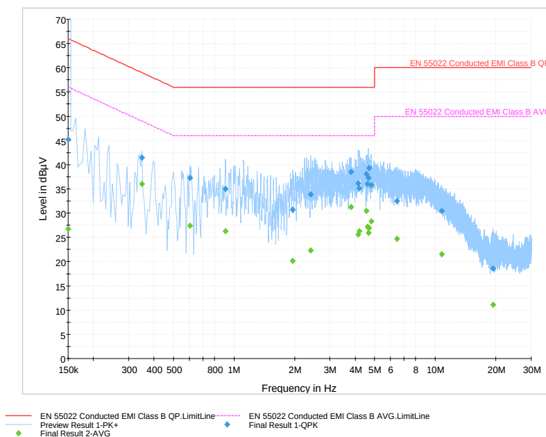
Figure 1-2: N Lines
