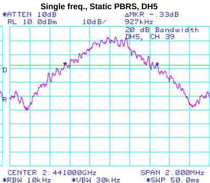
Figure 3-2: 20 dB Bandwidth
