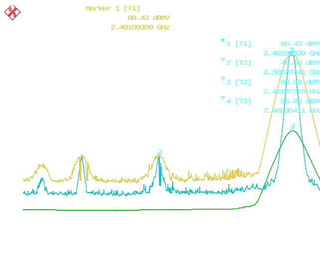
Figure 2-1: Band-Edge Compliance of RF Rad. Emissions. Bluetooth, Single freq., Static PBRS, DH5, Channel 0, Pol: V, Detector: PK
