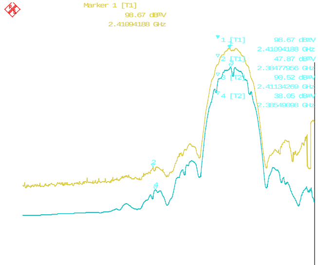
Figure 2-14: Band-Edge Compliance of RF Radiated Emission 802.11b, Channel 1, 2412 MHz, Max Pol: H, Detector: PK
