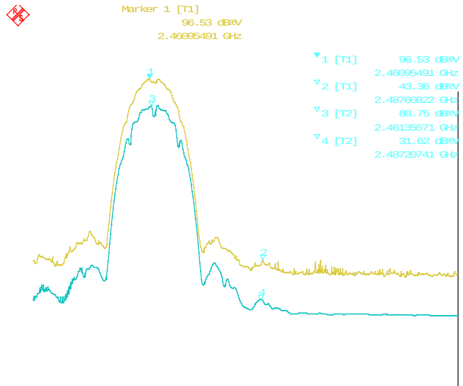
Figure 2-16: Band-Edge Compliance of RF Radiated Emission 802.11b, Channel 11, 2462 MHz, Max Pol: H, Detector: PK
