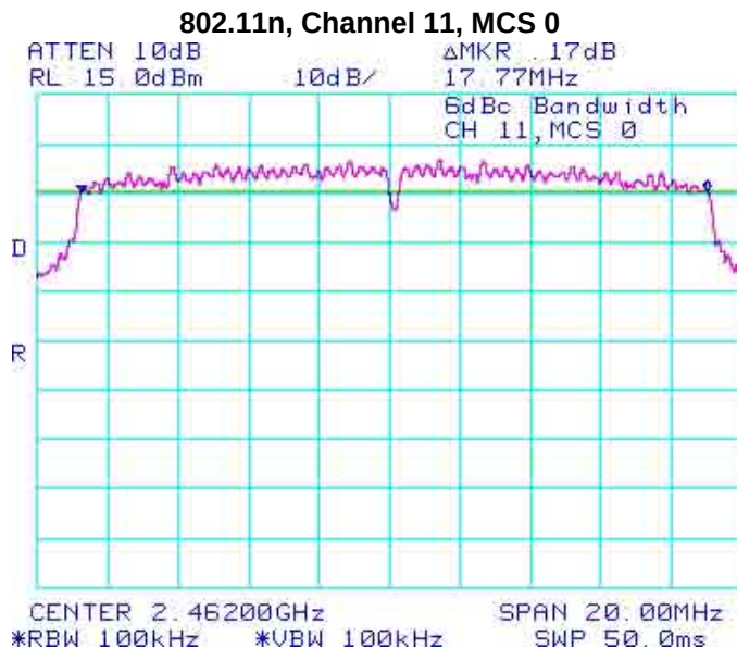
Figure 4-9: 6 dB Bandwidth
