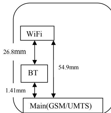
Figure 1.9.2. Back view of device showing closet distance between antenna pairs
