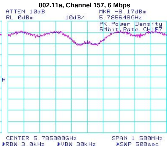
Figure 5-23: Peak Power Spectral Density
