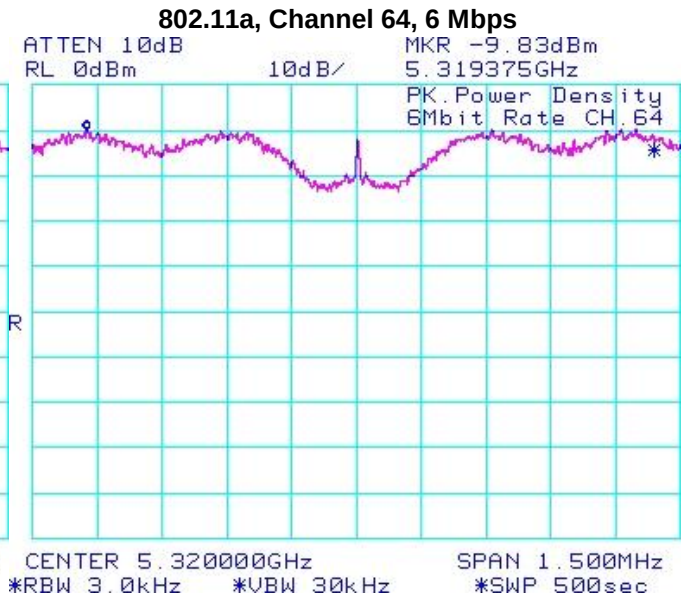
Figure 5-21: Peak Power Spectral Density
