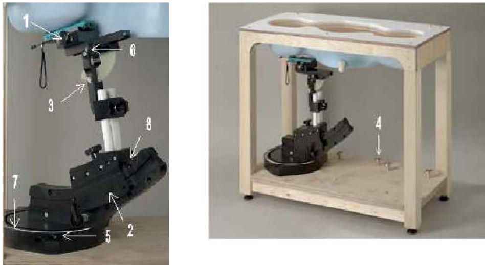
Figure 8.1.1. Device Holder
