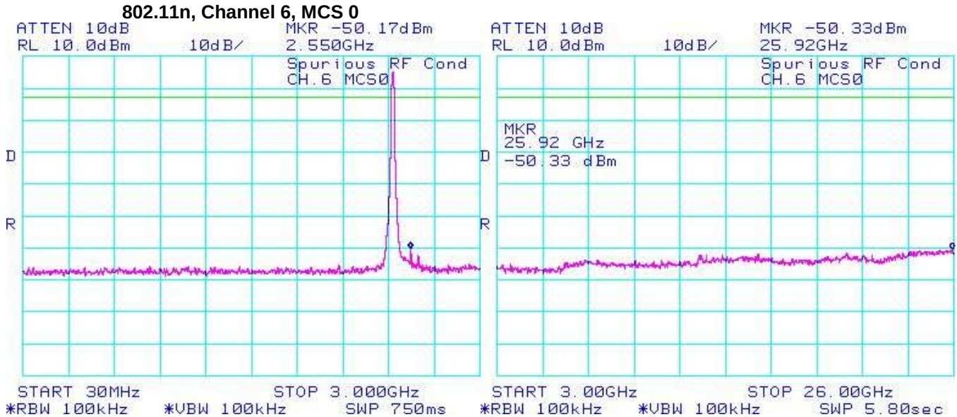
Figure 5-32: Spurious Conducted RF Emissions
