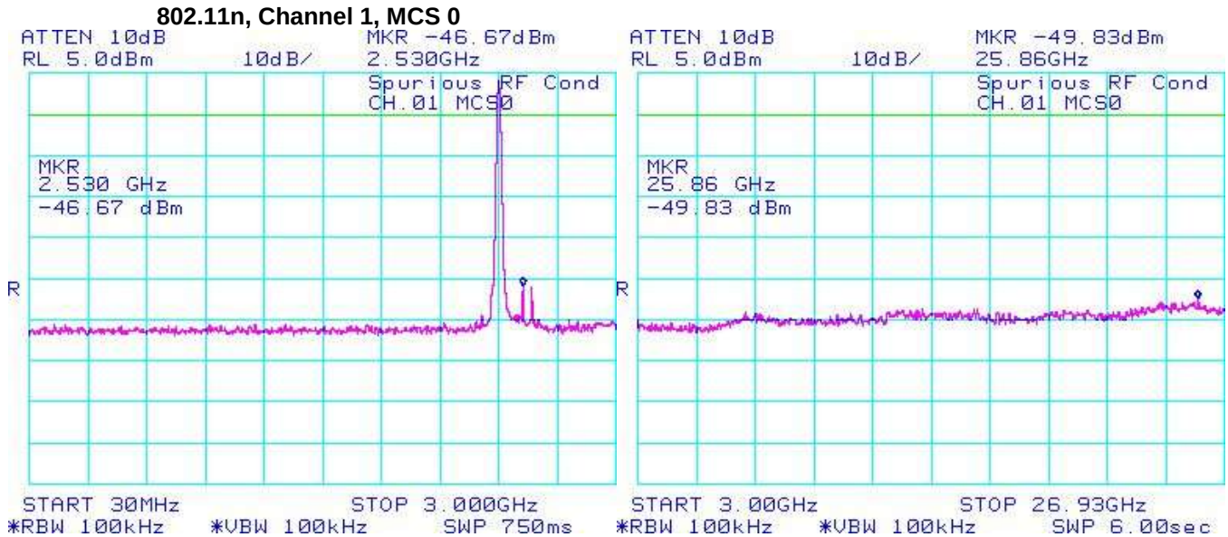
Figure 5-31: Spurious Conducted RF Emissions
