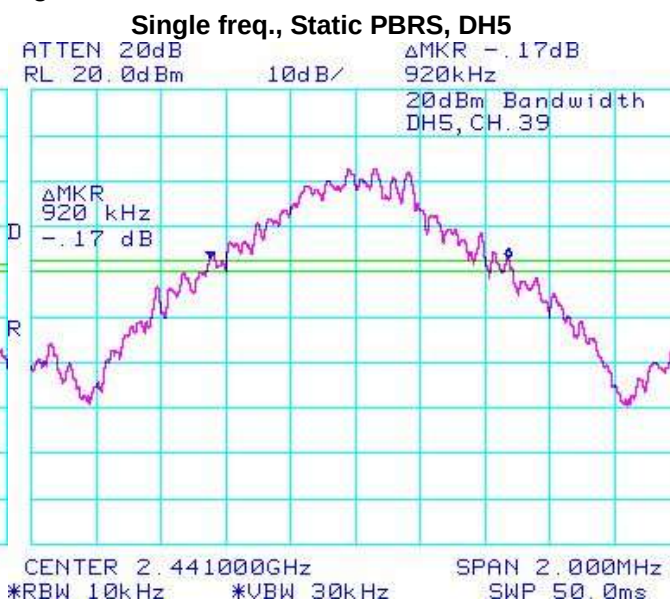
Figure 4-2: 20 dB Bandwidth
