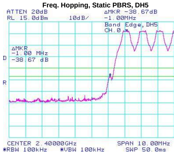
Figure 4-30: Band Edge Compliance
