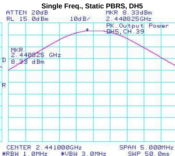
Figure 4-23: Max. Peak Conducted Output Power
