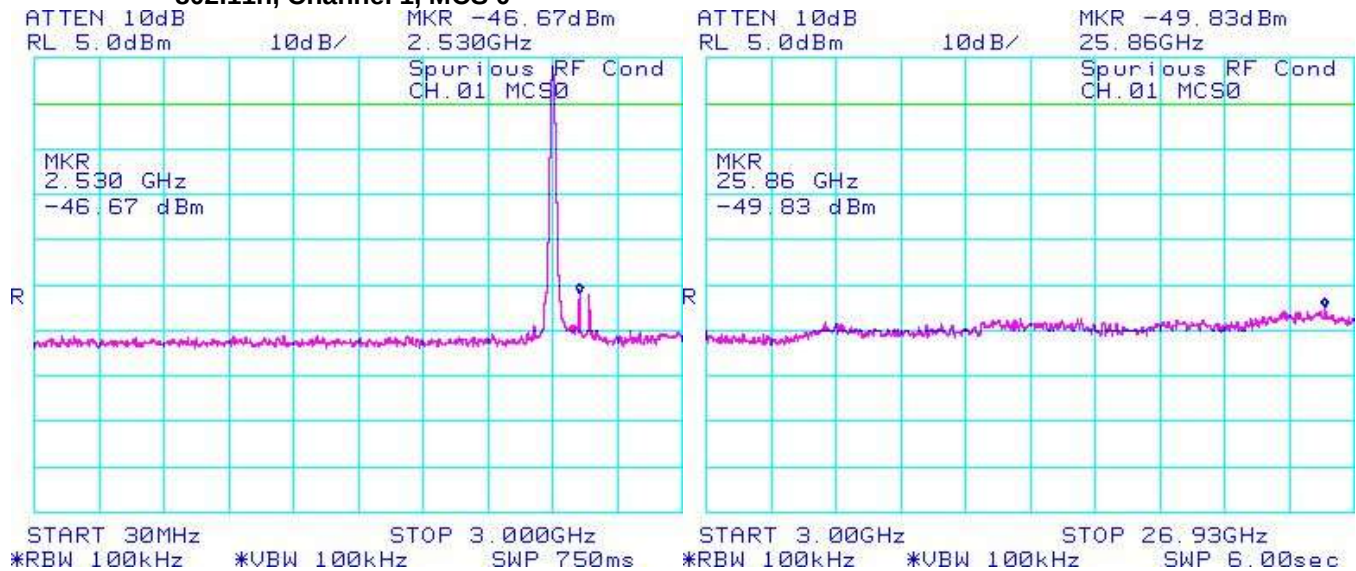
Figure 5-31: Spurious Conducted RF Emissions
