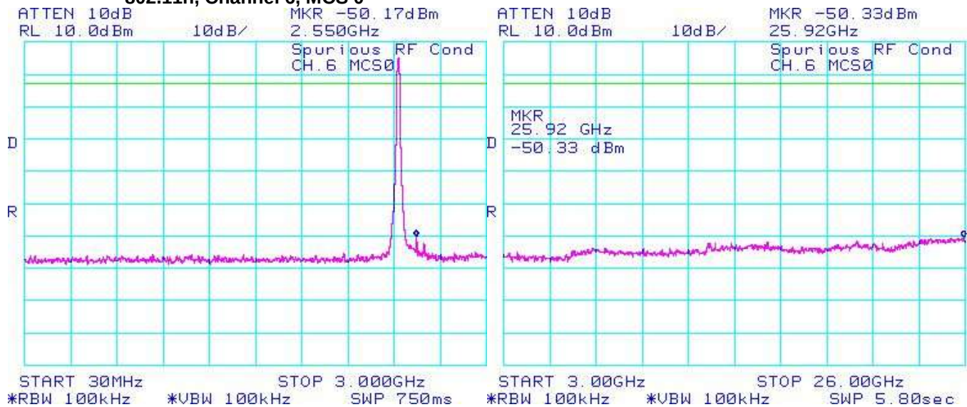
Figure 5-32: Spurious Conducted RF Emissions
