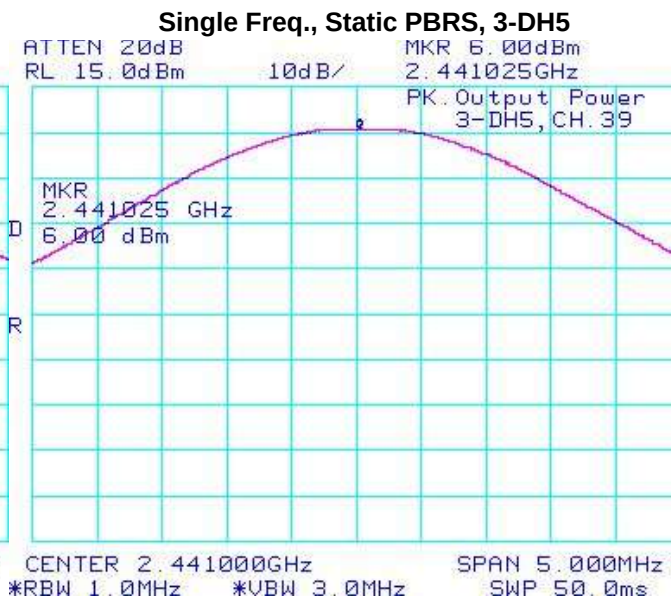
Figure 4-26: Max. Peak Conducted Output Power
