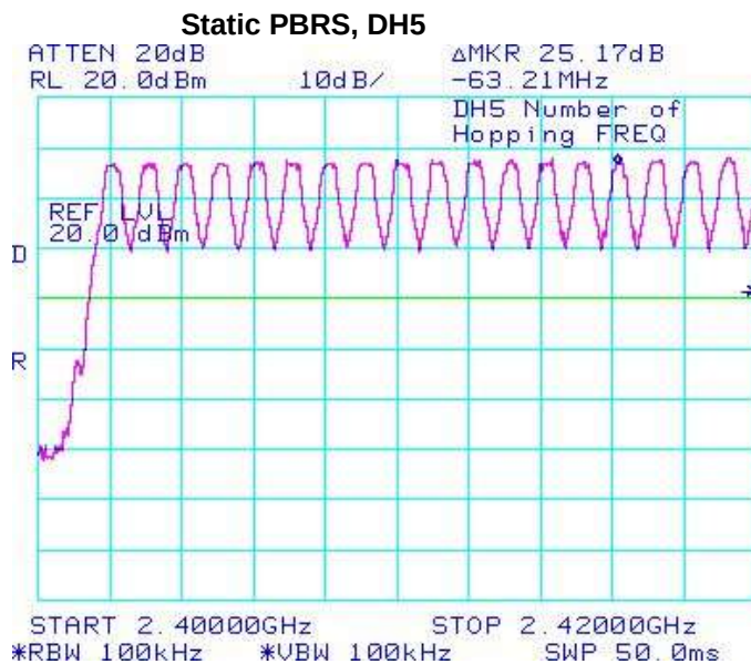
Figure 4-9: Number of Hopping Frequencies
