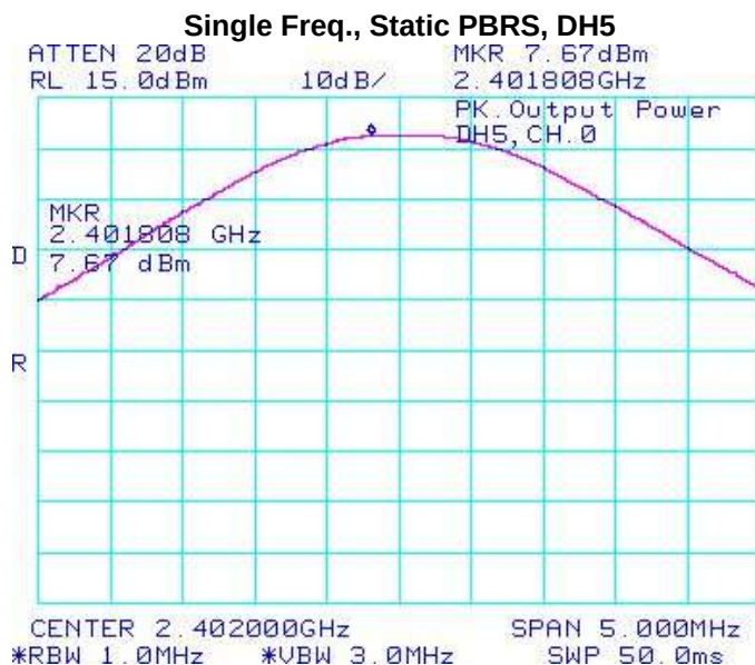
Figure 4-22: Max. Peak Conducted Output Power
