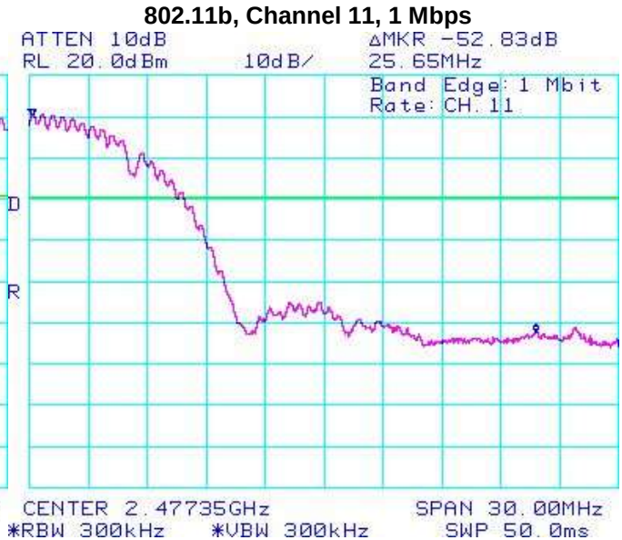
Figure 5-11: Band Edge Compliance
