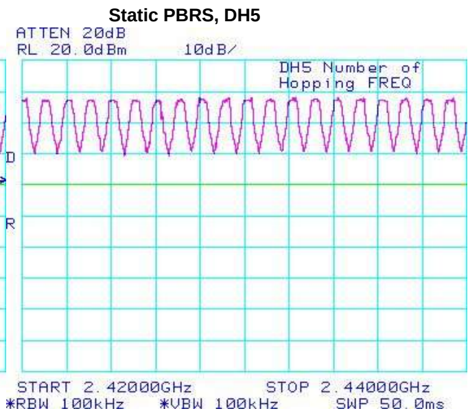
Figure 4-10: Number of Hopping Frequencies
