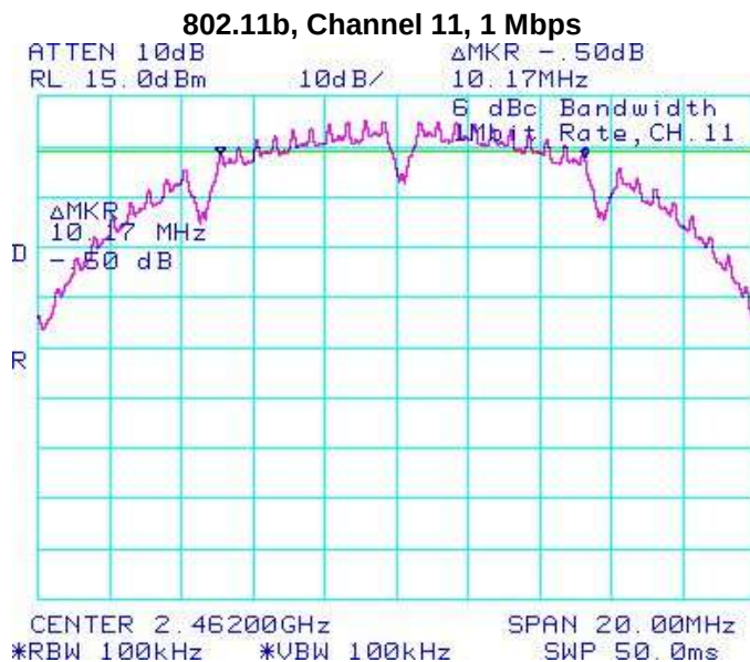
Figure 5-3: 6 dB Bandwidth
