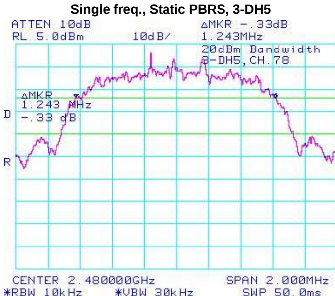
Figure 4-6: 20 dB Bandwidth
