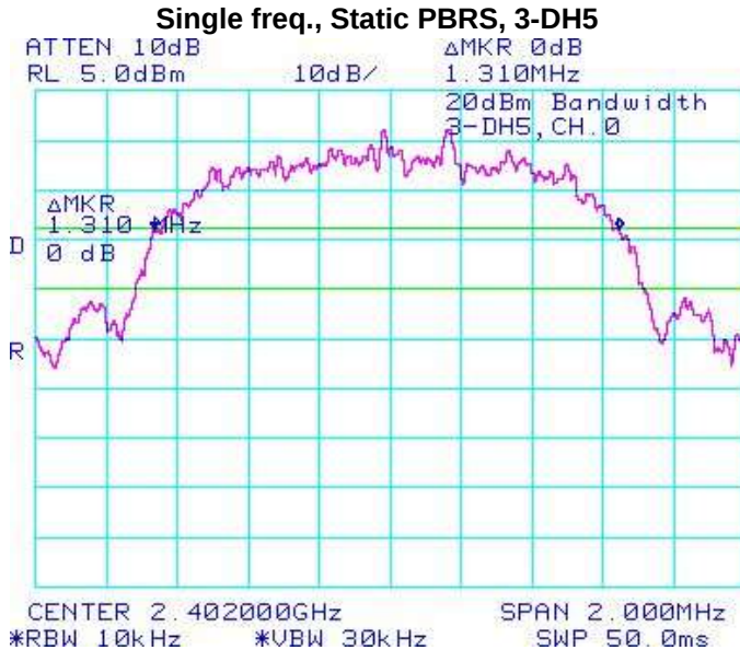
Figure 4-4: 20 dB Bandwidth
