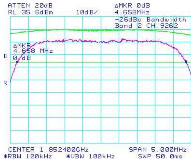
Figure 1-20c: -26 dBc Bandwidth, Band 2 Low Channel
