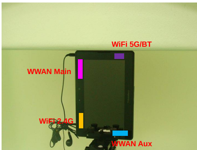
Primary Portrait to flat phantom with 0 cm gap
