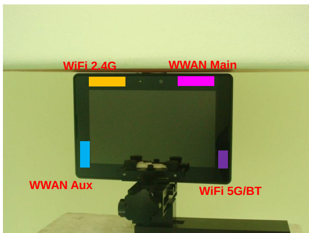
Secondary Landscape to flat phantom with 0 cm gap
