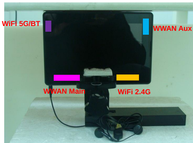
Primary Landscape to flat phantom with 0 cm gap
