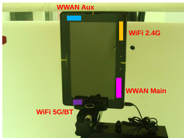
Secondary Portrait to flat phantom with 0 cm gap
