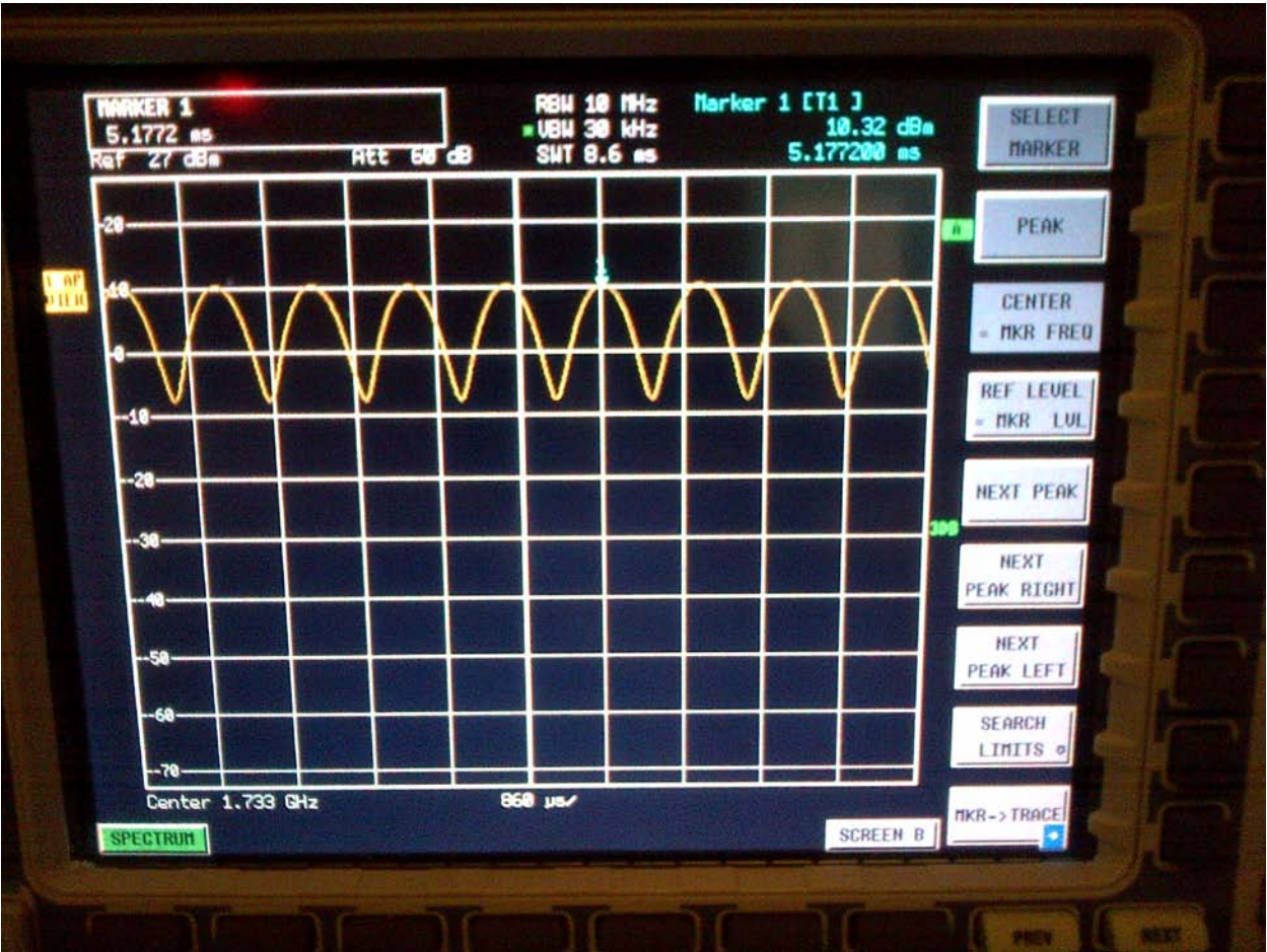
AM80% 1733 MHz
