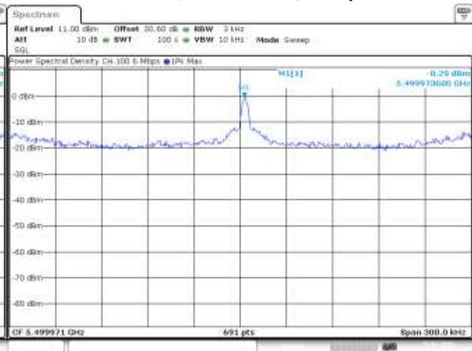
Figure 6-25: Peak Power Spectral Density 802.11a, Channel 100, 6 Mbps
