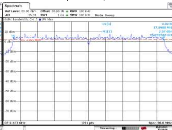
Figure 5-8: 6 dB Bandwidth 802.11n, Channel 6, MCS 0
