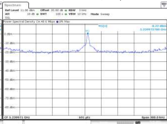
Figure 6-23: Peak Power Spectral Density 802.11a, Channel 48, 6 Mbps
