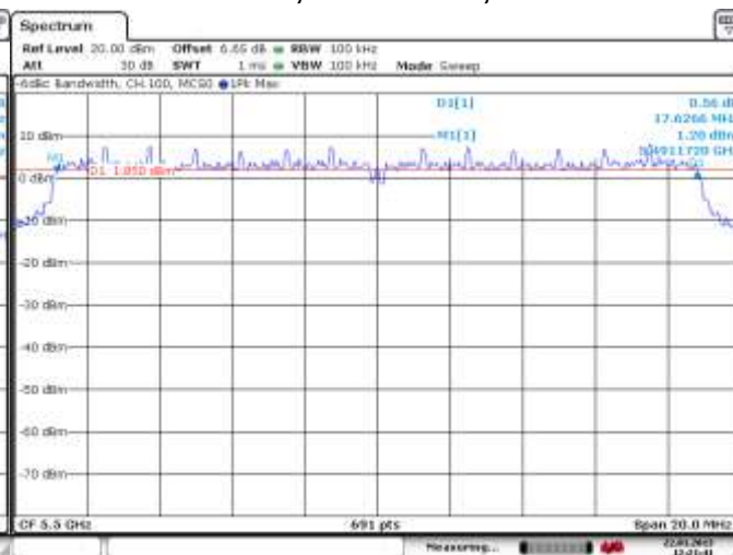
Figure 6-8: 6 dB Bandwidth 802.11n, Channel 100, MCS 0
