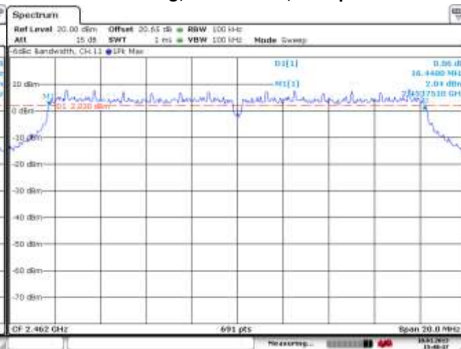
Figure 5-6: 6 dB Bandwidth 802.11g, Channel 11, 6 Mbps
