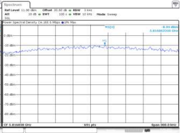
Figure 6-27: Peak Power Spectral Density 802.11a, Channel 165, 6 Mbps
