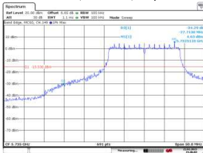
Figure 6-20: Band Edge Compliance 802.11n, Channel 149, 6 Mbps
