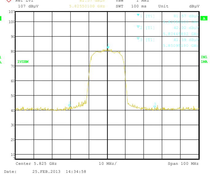
Figure 3-14: Band-Edge Compliance of RF Radiated Emission. 802.11a, Ch 165, 5825 MHz, Centre of Band-Edge: 5805 MHz
