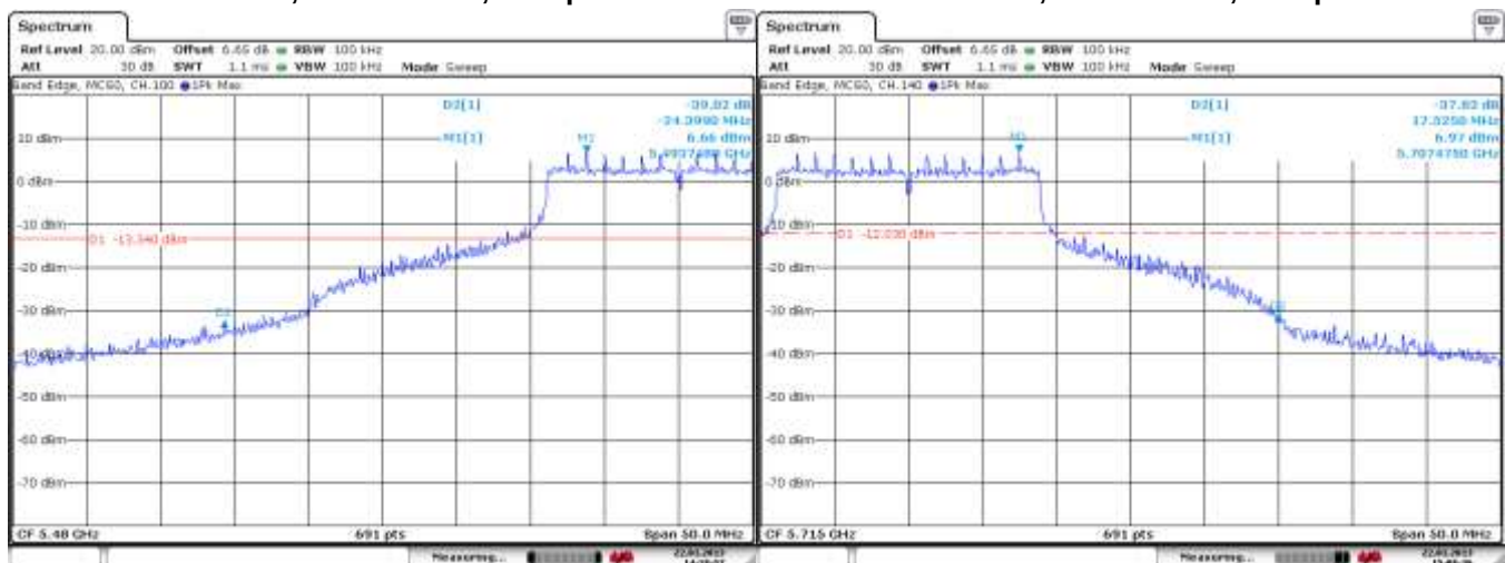
Figure 6-24: Band Edge Compliance 802.11n, Channel 100, 6 Mbps
