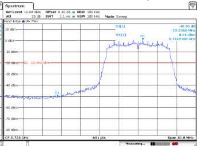
Figure 6-20: Band Edge Compliance 802.11a, Channel 149, 6 Mbps
