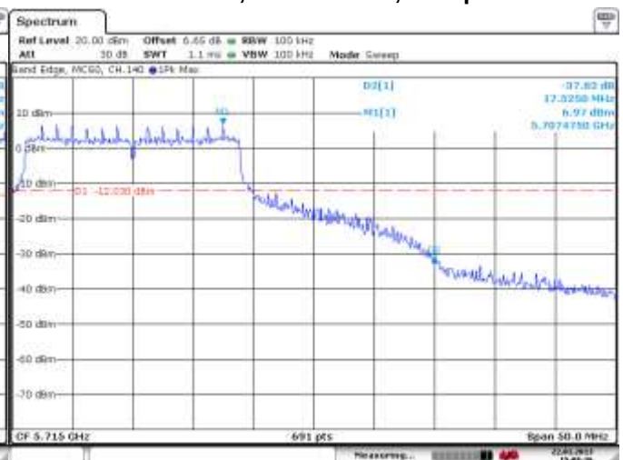
Figure 6-25: Band Edge Compliance 802.11n, Channel 140, 6 Mbps
