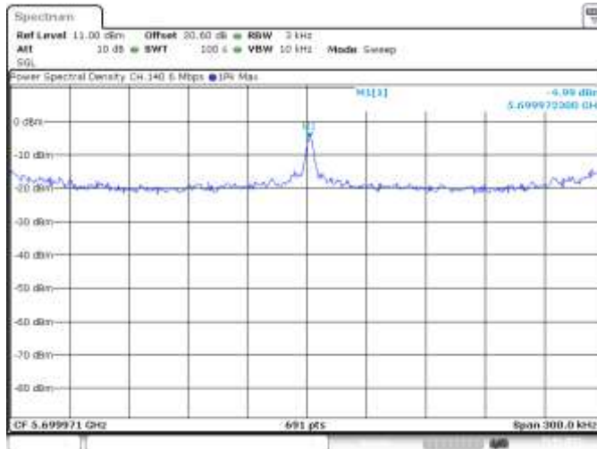
Figure 6-32: Peak Power Spectral Density 802.11a, Channel 140, 6 Mbps
