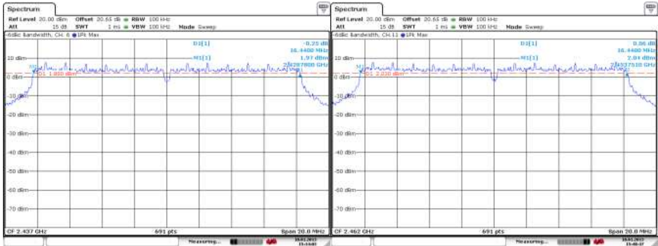
Figure 5-5: 6 dB Bandwidth 802.11g, Channel 6, 6 Mbps
