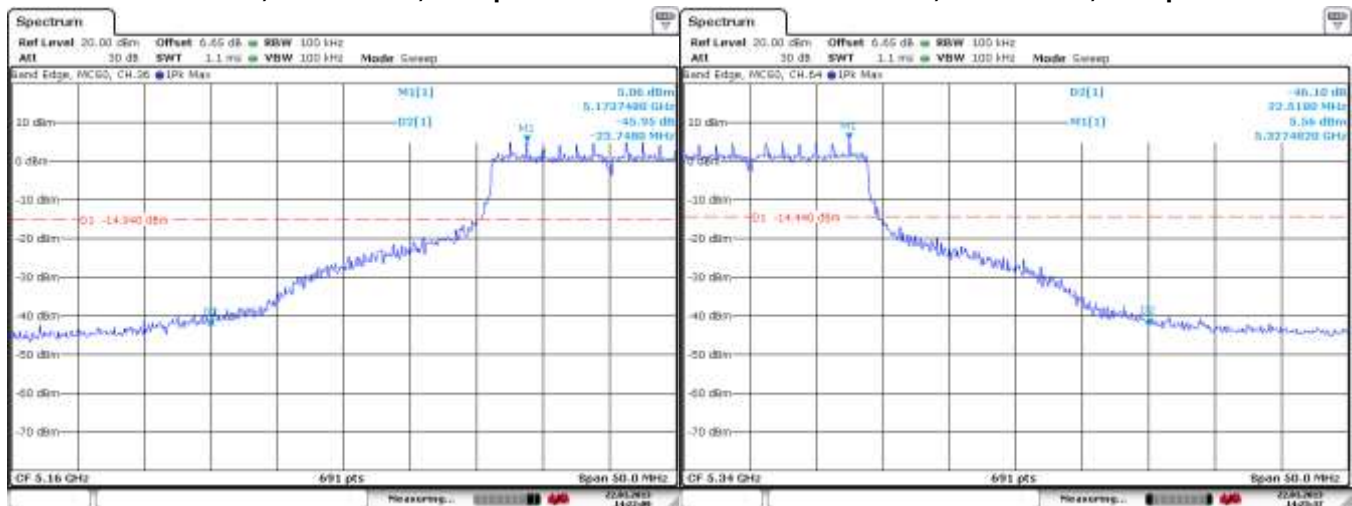
Figure 6-22: Band Edge Compliance 802.11n, Channel 36, 6 Mbps
