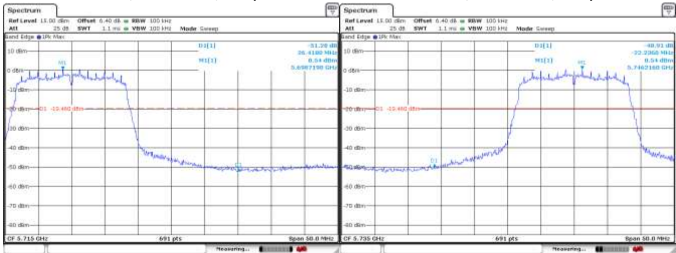
Figure 6-19: Band Edge Compliance 802.11a, Channel 140, 6 Mbps
