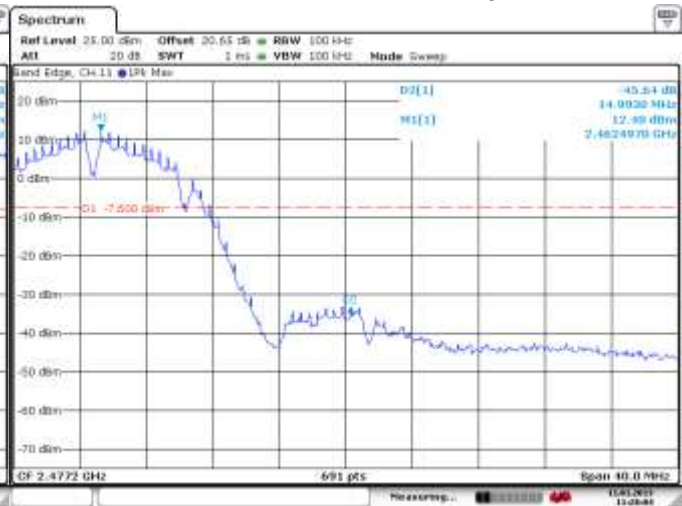
Figure 5-11: Band Edge Compliance 802.11b, Channel 11, 1 Mbps
