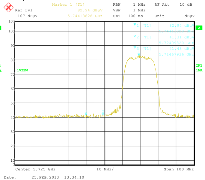
Figure 3-10: Band-Edge Compliance of RF Radiated Emission. 802.11a, Ch 149, 5745 MHz, Centre of Band-Edge: 5725 and 5715 MHz
