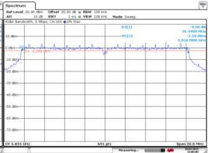
Figure 6-6: 6 dB Bandwidth 802.11a, Channel 165, 6 Mbps
