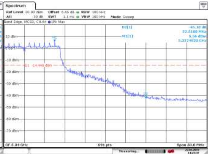
Figure 6-14: Band Edge Compliance 802.11a, Channel 64, 6 Mbps
