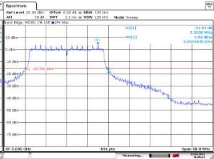
Figure 6-27: Band Edge Compliance 802.11n, Channel 165, 6 Mbps
