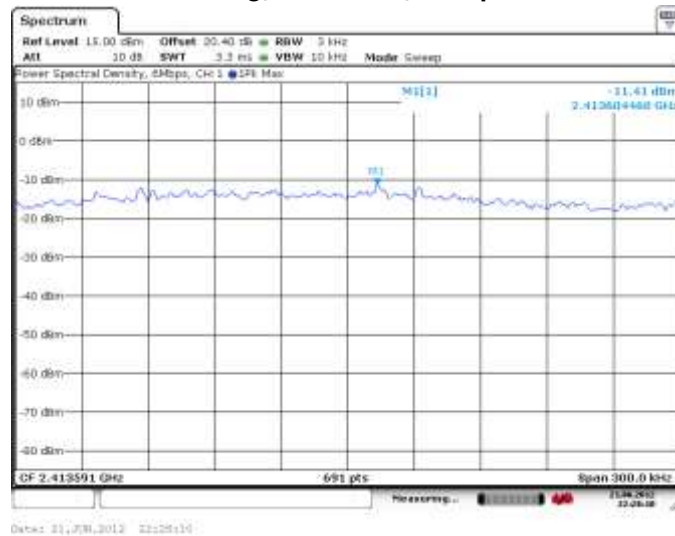
Figure 5-22: Peak Power Spectral Density 802.11g, Channel 1, 6 Mbps
