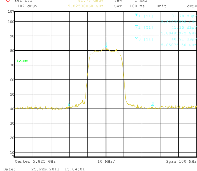
Figure 3-13: Band-Edge Compliance of RF Radiated Emission 802.11a, Ch 165, 5825 MHz, Centre of Band-Edge: 5805 MHz
