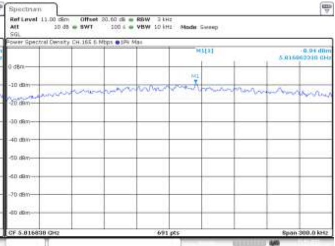
Figure 6-33: Peak Power Spectral Density 802.11a, Channel 165, 6 Mbps
