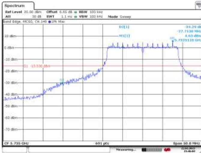
Figure 6-26: Band Edge Compliance 802.11n, Channel 149, 6 Mbps
