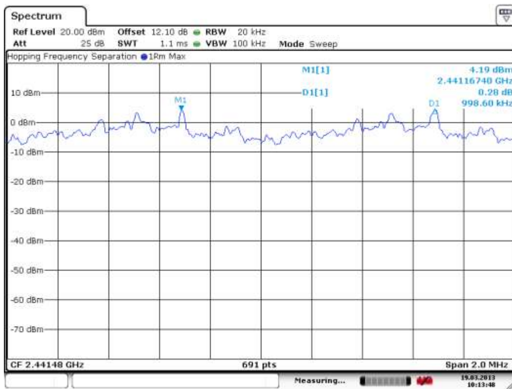
Figure 4-12: Carrier Frequency Separation, Freq. Hopping, Static PBRs, 3-DH5, Channels 38 to 39
