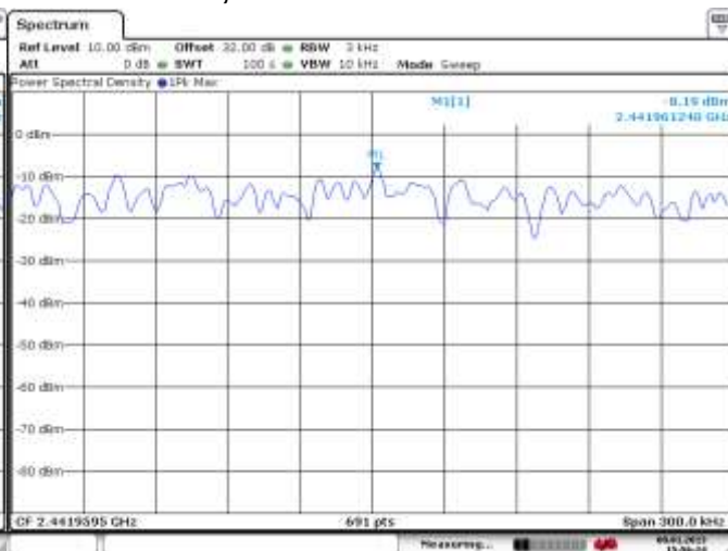
Figure 4-65: Peak Power Spectral Density LE, Channel 20
