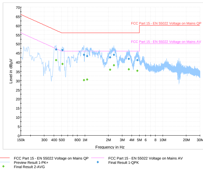
Figure 1-10: N Lines
