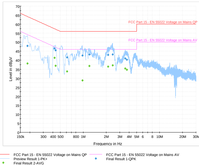
Figure 1-10: N Lines
