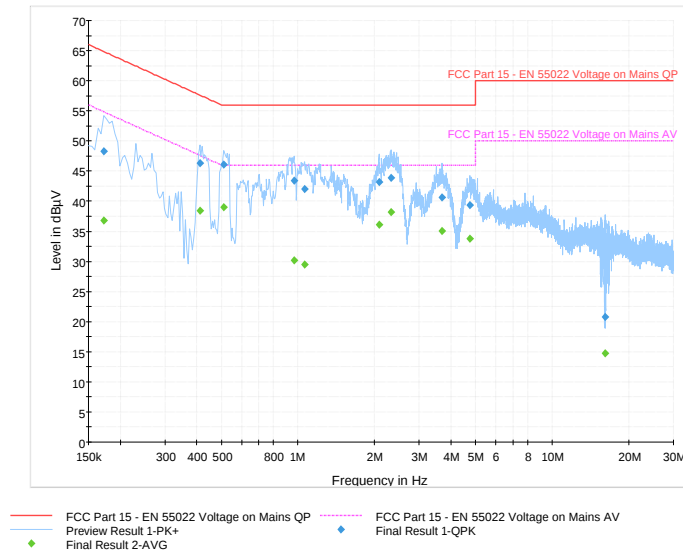
Figure 1-15: L1 lines
