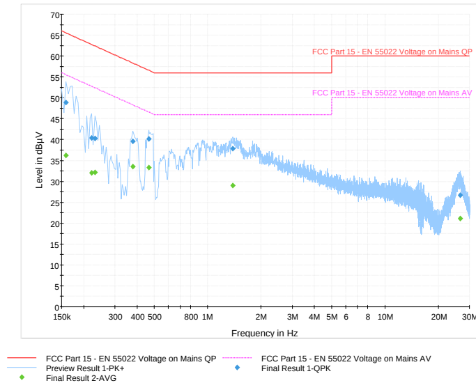
Figure 1-19: L1 lines
