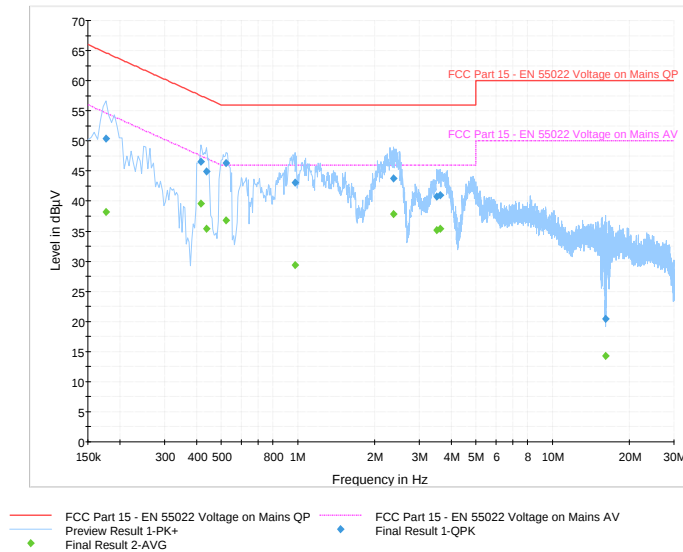
Figure 1-17: L1 lines
