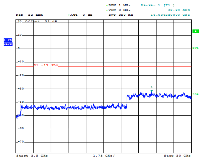
Figure 1-12b: BAND 2, Spurious Conducted Emissions, High Channel
