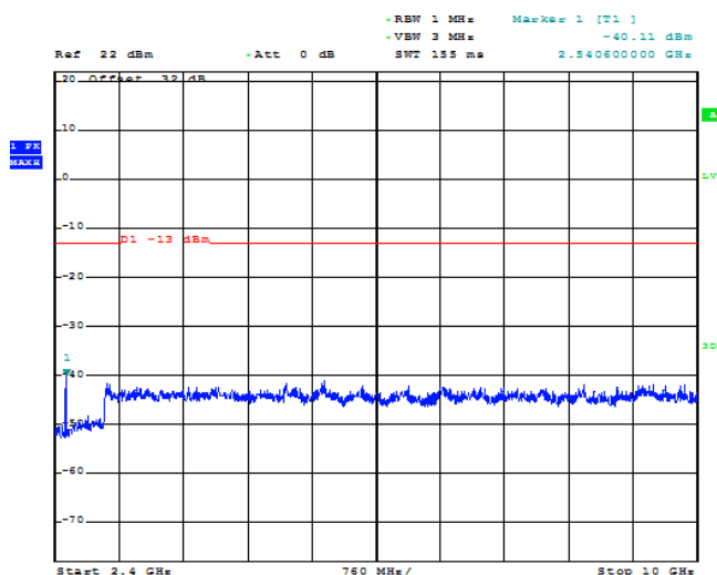
Figure 1-6b: Band 5, Spurious Conducted Emissions, High Channel
