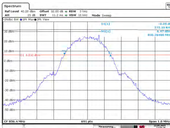
Figure 1-14a: -26dBc bandwidth, GSM850 band Middle Channel in GSM mode
