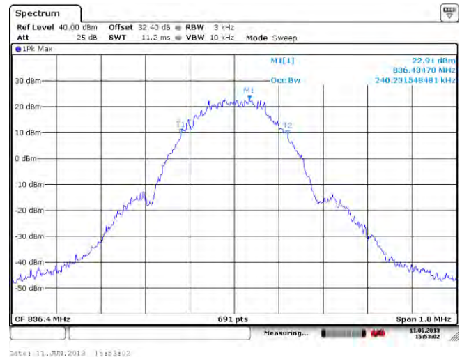
Figure 1-33a: Occupied Bandwidth, GSM850 Band, Middle Channel in EDGE mode
