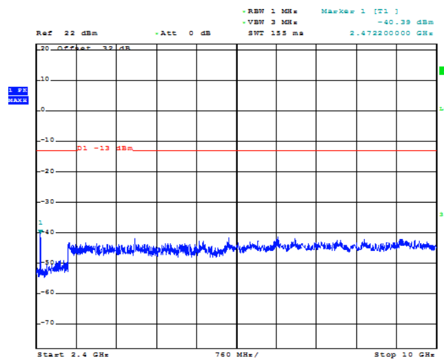
Figure 1-33b: Band 5 HSUPA, Spurious Conducted Emissions, Low channel
