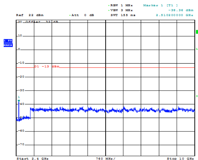
Figure 1-35b: Band 5 HSUPA, Spurious Conducted Emissions, Middle channel
