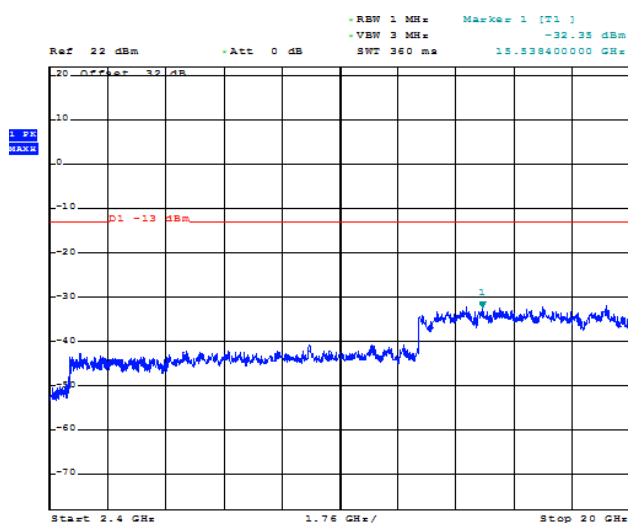
Figure 1-39b: Band 2 HSUPA, Spurious Conducted Emissions, Low Channel
