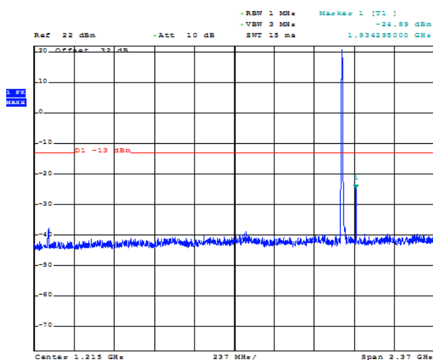
Figure 1-38b: Band 2 HSUPA, Spurious Conducted Emissions, Low Channel
