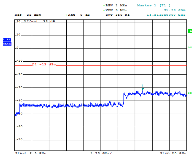
Figure 1-8b: BAND 2, Spurious Conducted Emissions, Low Channel
