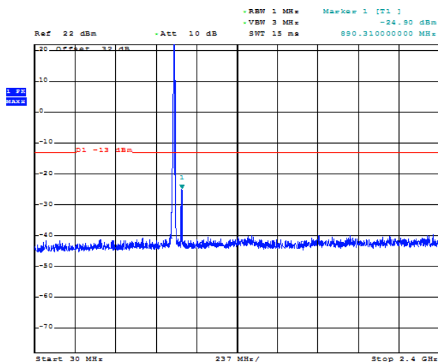
Figure 1-36b: Band 5 HSUPA, Spurious Conducted Emissions, High Channel
