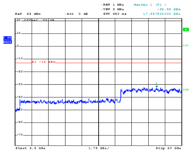
Figure 1-10b: BAND 2, Spurious Conducted Emissions, Middle Channel
