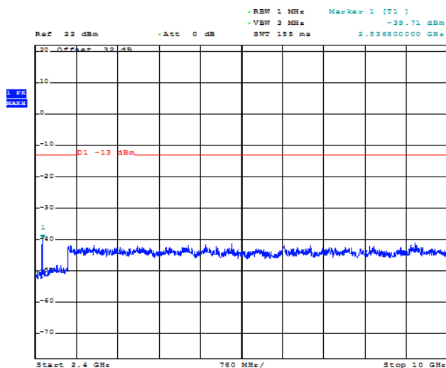
Figure 1-37b: Band 5 HSUPA, Spurious Conducted Emissions, High Channel
