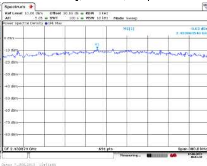
Figure 2-20: Peak Power Spectral Density 802.11g, Channel 6, 6 Mbps
