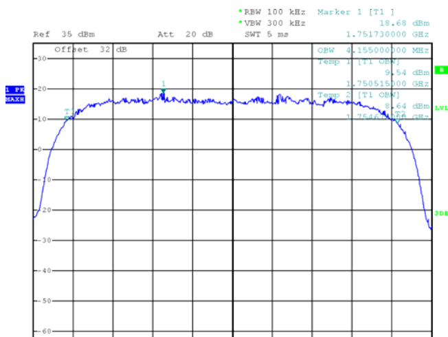
Figure 2-9b: Occupied Bandwidth, Band IV High Channel
