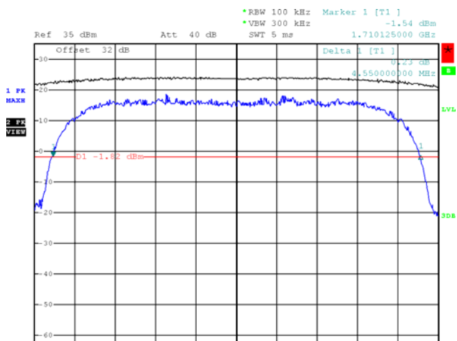
Figure 2-10b: -26 dBc Bandwidth, Band IV Low Channel
