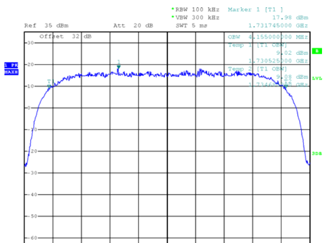
Figure 2-8b: Occupied Bandwidth, Band IV Middle Channel
