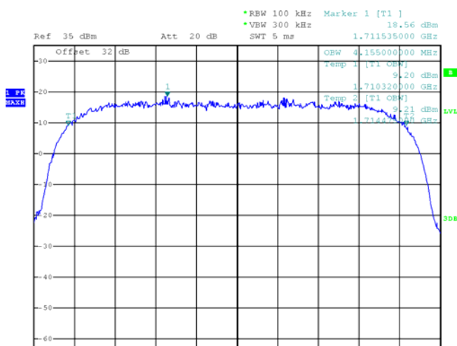
Figure 2-7b: Occupied Bandwidth, Band IV Low Channel
