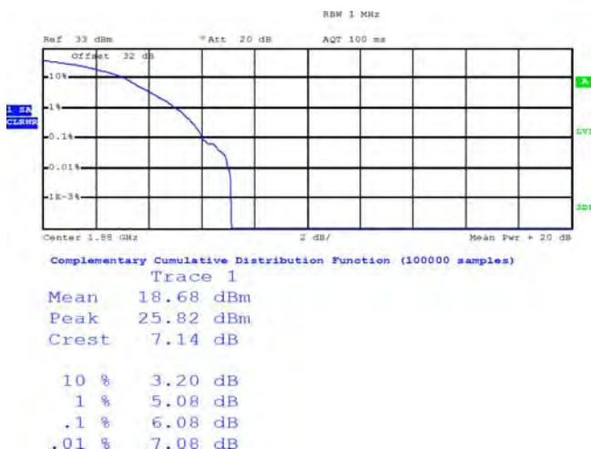
Figure 3-42a: Band 2, Mid Channel PAR, 1.4 MHz BW, RB = 6 16-QAM
