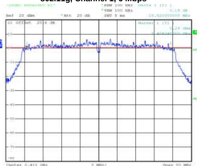
Figure 3-4: 6 dB Bandwidth 802.11g, Channel 1, 6 Mbps
