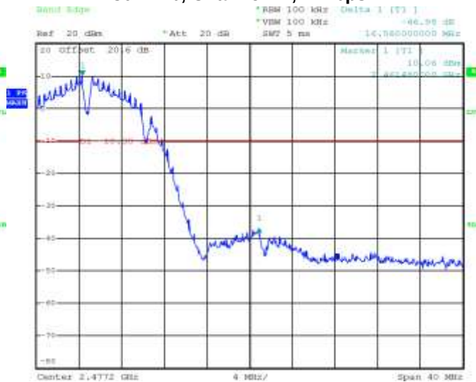
Figure 3-11: Band Edge Compliance 802.11b, Channel 11, 1 Mbps
