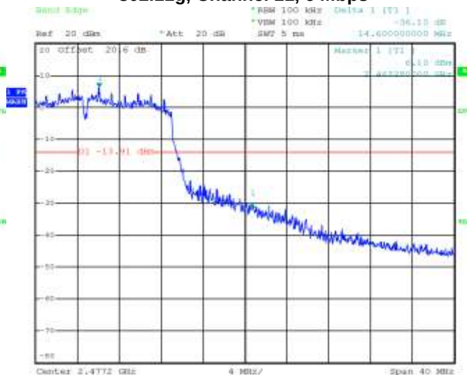
Figure 3-13: Band Edge Compliance 802.11g, Channel 11, 6 Mbps
