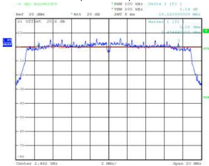
Figure 3-9: 6 dB Bandwidth 802.11n, Channel 11, MCS 0
