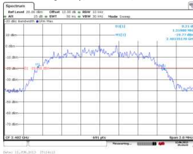
Figure 2-4: 20 dB Bandwidth Single freq., Static PBRS, 2-DH5
