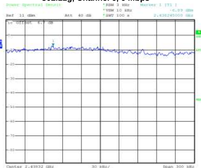
Figure 3-20: Peak Power Spectral Density 802.11g, Channel 6, 6 Mbps
