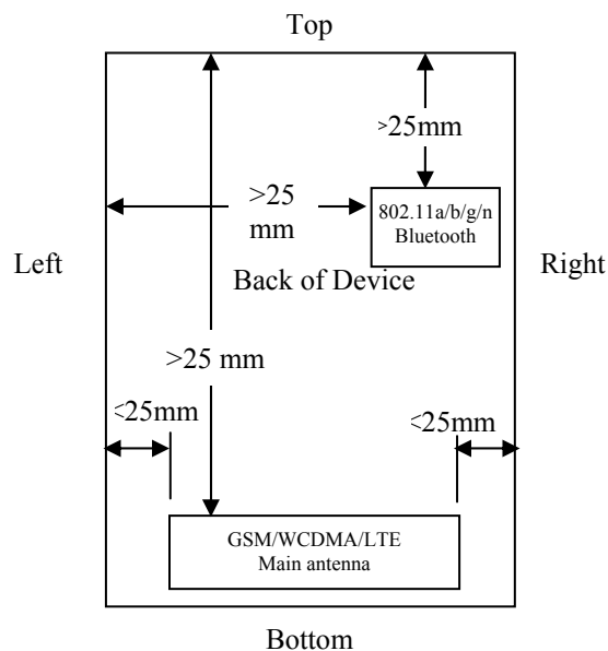
Figure 1.8.2-1 Identification of all sides for SAR Testing
