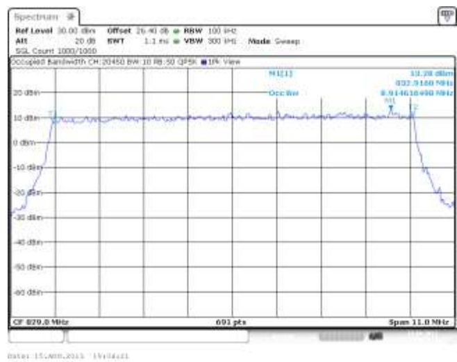
Figure 3-19a: Occupied Bandwidth, Band 5 Low Channel, 10MHz BW, RB=50
