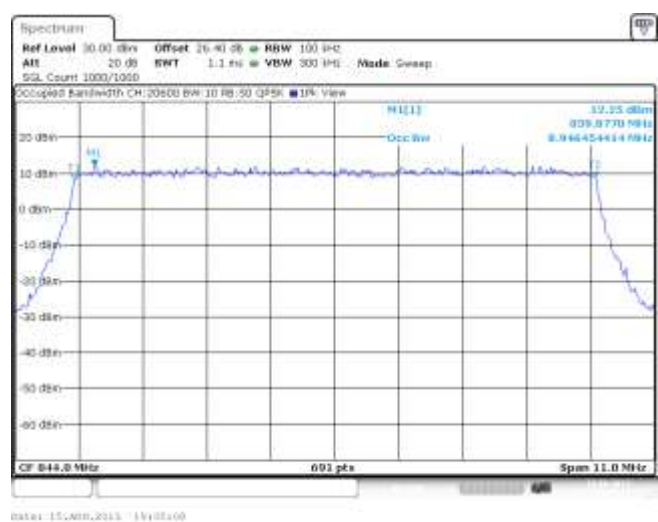
Figure 3-21a: Occupied Bandwidth, Band 5 High Channel, 10MHz BW, RB=50
