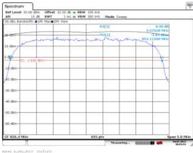
Figure 2-19a: -26 dBc Bandwidth, Band 5 Low Channel
