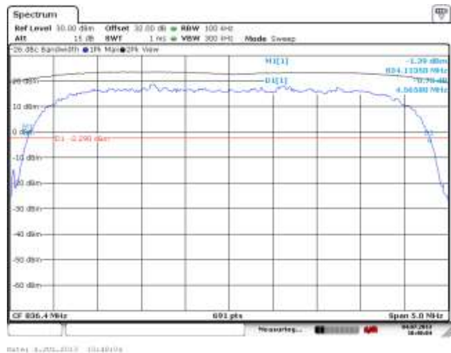
Figure 2-20a: -26 dBc Bandwidth, Band 5 Middle Channel
