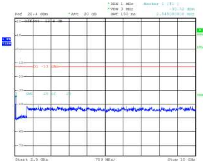
Figure 3-18a: Band 5, Spurious Conducted Emissions, High channel, 1.4MHz BW (RB= 6)
