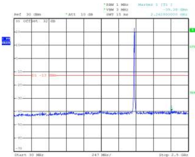
Figure 2-3b: Band 4, Spurious Conducted Emissions, Middle channel
