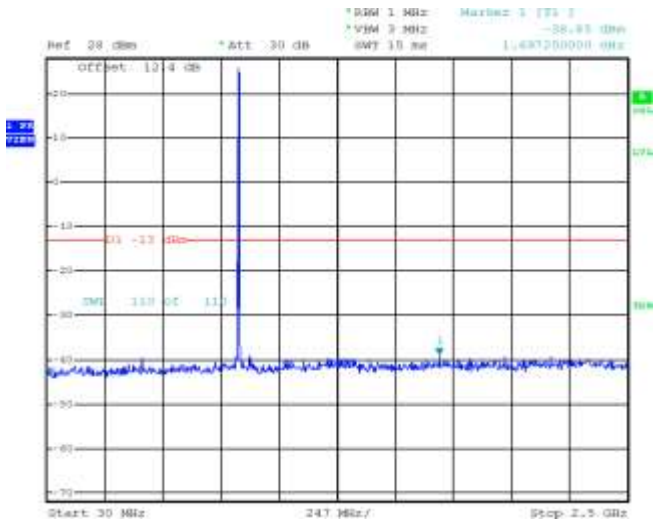
Figure 3-17a: Band 5, Spurious Conducted Emissions, High channel, 1.4MHz BW (RB= 6)
