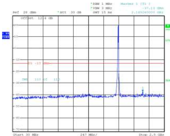
Figure 4-11a: Band 4, Spurious Conducted Emissions, High channel, 10MHz BW (RB= 50)
