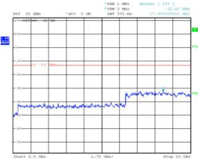
Figure 2-6b: Band 4, Spurious Conducted Emissions, High Channel
