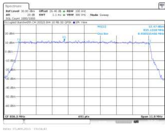
Figure 3-20a: Occupied Bandwidth, Band 5 Middle Channel, 10MHz BW, RB=50
