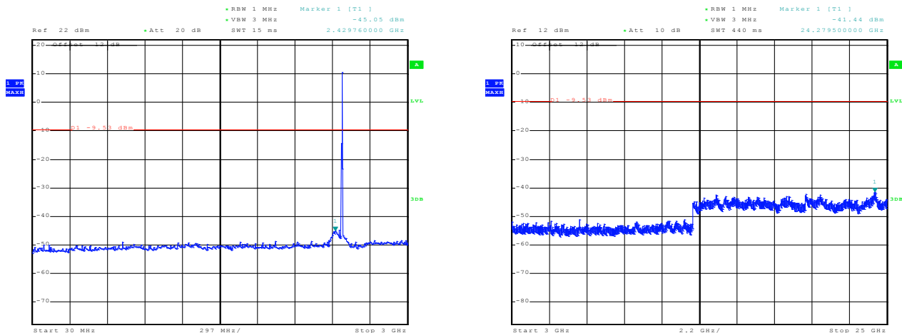
Figure 2-49: Spurious RF Conducted Emissions Single Freq., Static PBRS, DH5
