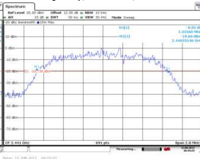
Figure 2-8: 20 dB Bandwidth Single freq., Static PBRs, 3-DH5
