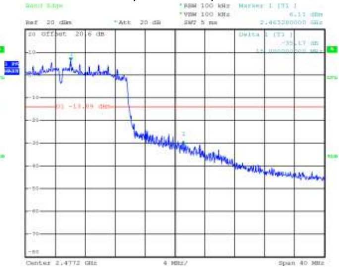
Figure 3-15: Band Edge Compliance 802.11n, Channel 11, MCS 0
