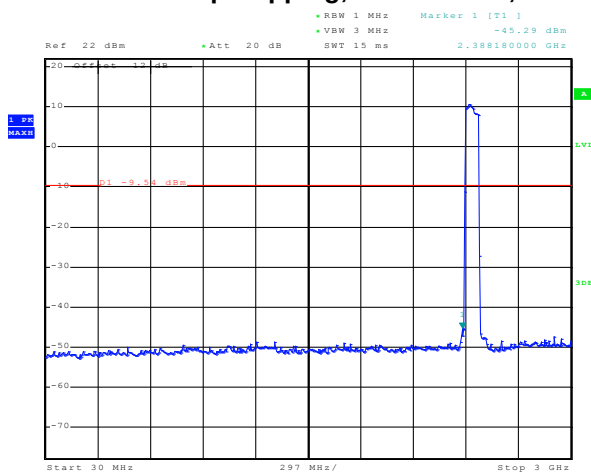
Figure 2-54: Spurious RF Conducted Emissions Freq. Hopping, Static PBRS, 2-DH5
