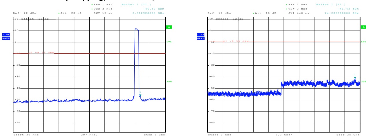
Figure 2-50: Spurious RF Conducted Emissions Freq. Hopping, Static PBRS, DH5
