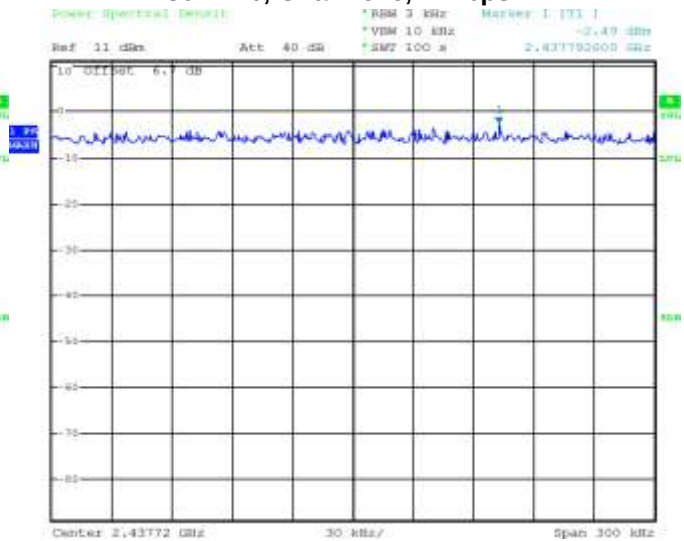
Figure 3-17: Peak Power Spectral Density 802.11b, Channel 6, 1 Mbps
