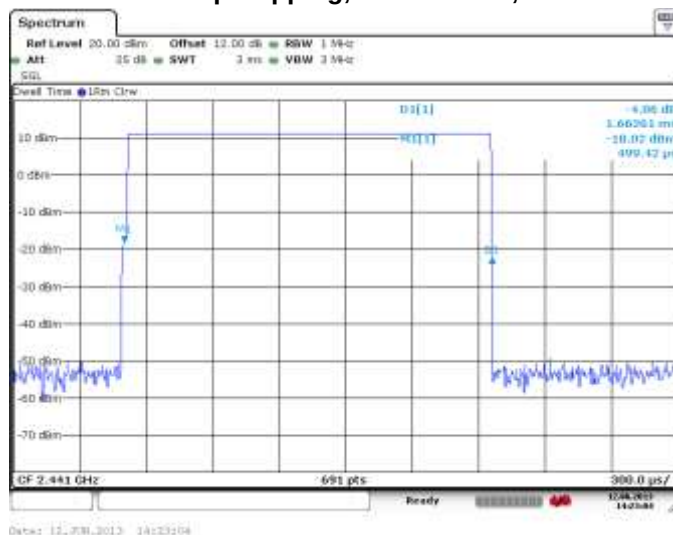
Figure 2-21: Time of Occupancy (Dwell Time) Freq. Hopping, Static PBRS, DH3
