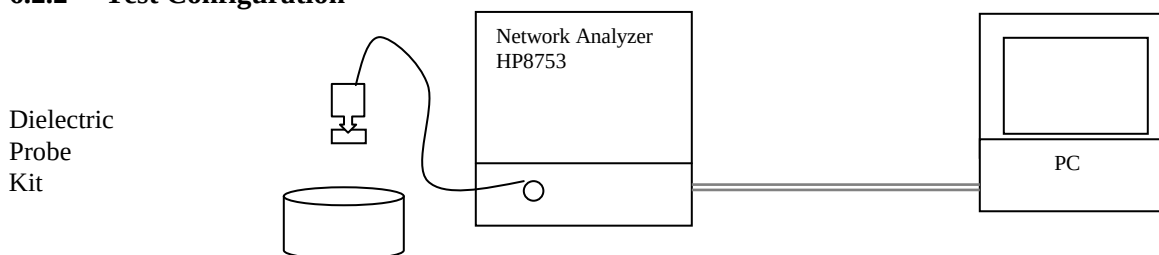
Figure 6.2.2-1 Test configuration
