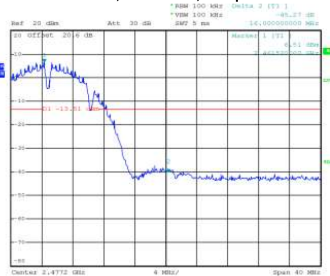
Figure 3-11: Band Edge Compliance
