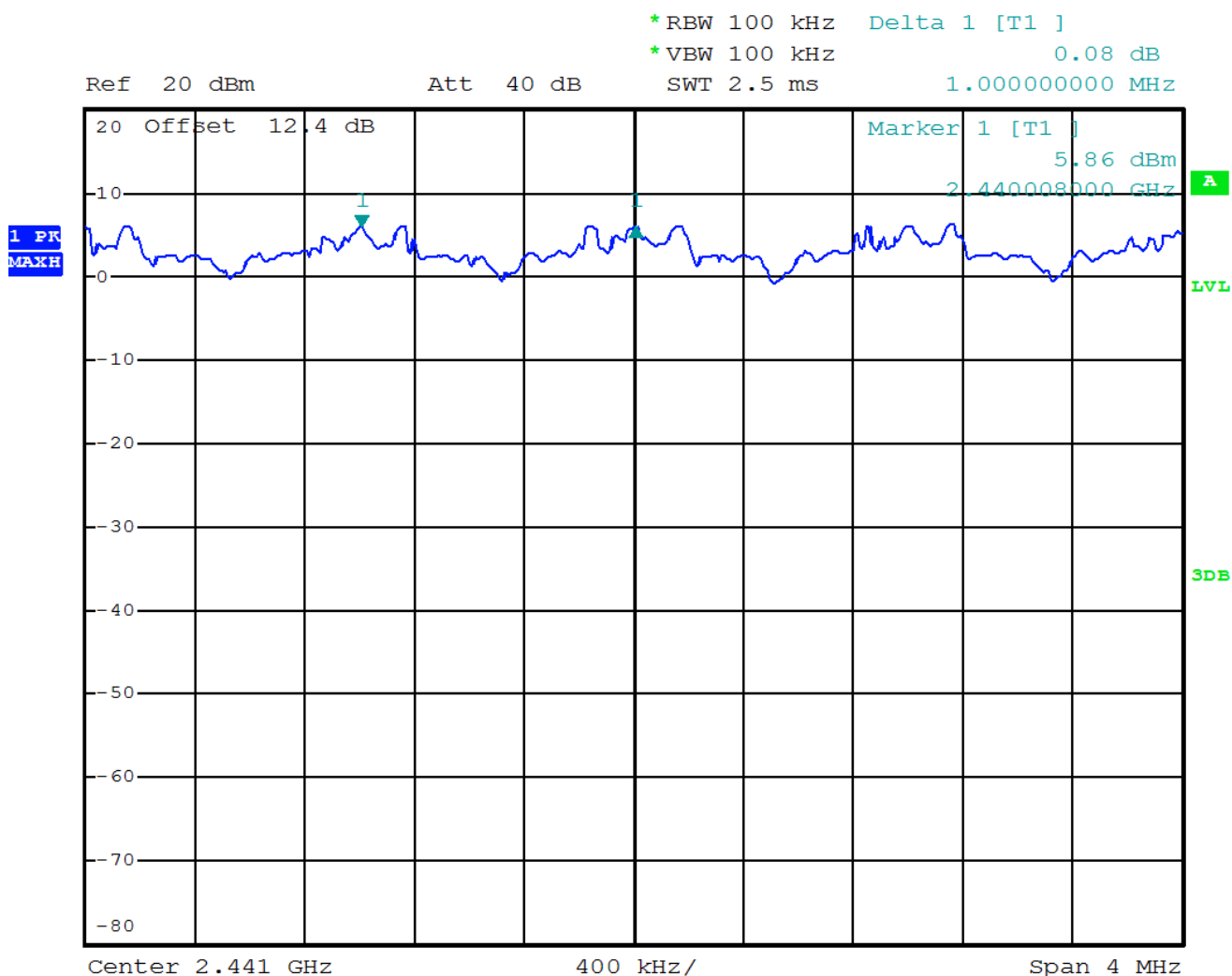
Figure 2-12: Carrier Frequency Separation, Freq. Hopping, Static PBRS, 3-DH5, Channels 38 to 39
