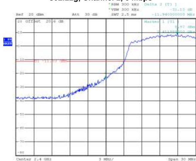
Figure 3-12: Band Edge Compliance
