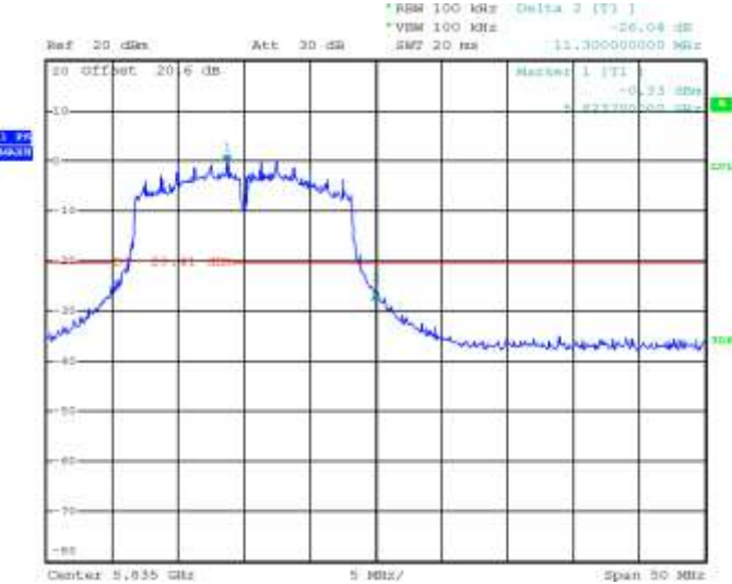
Figure 4-15: Band Edge Compliance 802.11a, Channel 165, 6 Mbps
