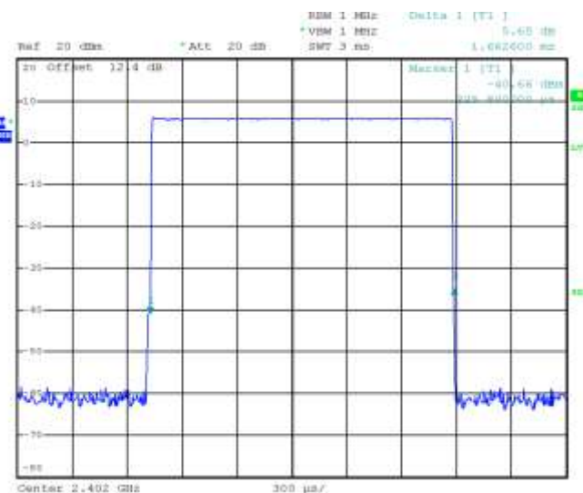
Figure 2-20: Time of Occupancy (Dwell Time) Freq. Hopping, Static PBRS, DH3
