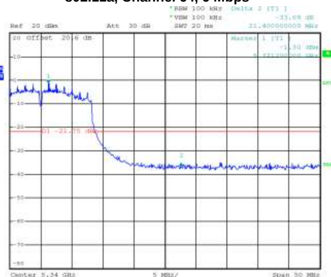
Figure 4-11: Band Edge Compliance 802.11a, Channel 64, 6 Mbps
