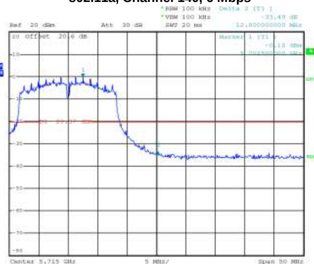
Figure 4-13: Band Edge Compliance 802.11a, Channel 140, 6 Mbps
