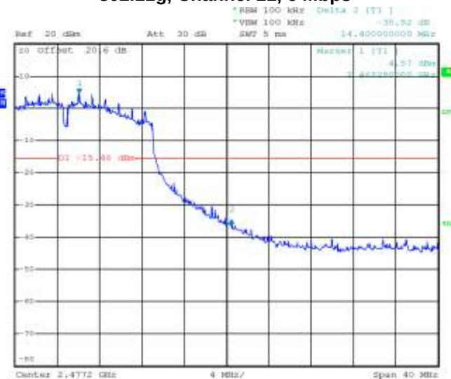
Figure 3-13: Band Edge Compliance
