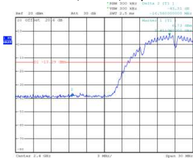
Figure 3-10: Band Edge Compliance
