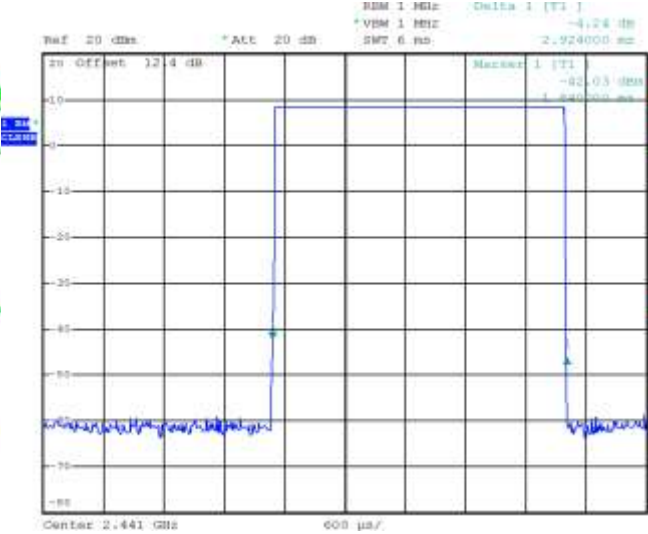
Figure 2-24: Time of Occupancy (Dwell Time) Freq. Hopping, Static PBRs, DH5
