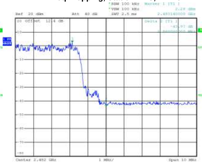
Figure 2-42: Band Edge Compliance Freq. Hopping, Static PBRS, 2-DH5
