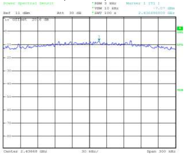
Figure 3-23: Peak Power Spectral Density 802.11n, Channel 6, MCS 0
