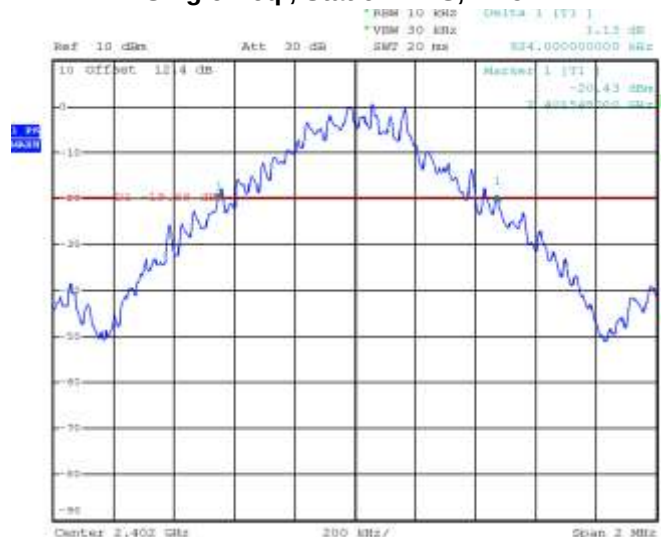
Figure 2-1: 20 dB Bandwidth Single freq., Static PBRS, DH5
