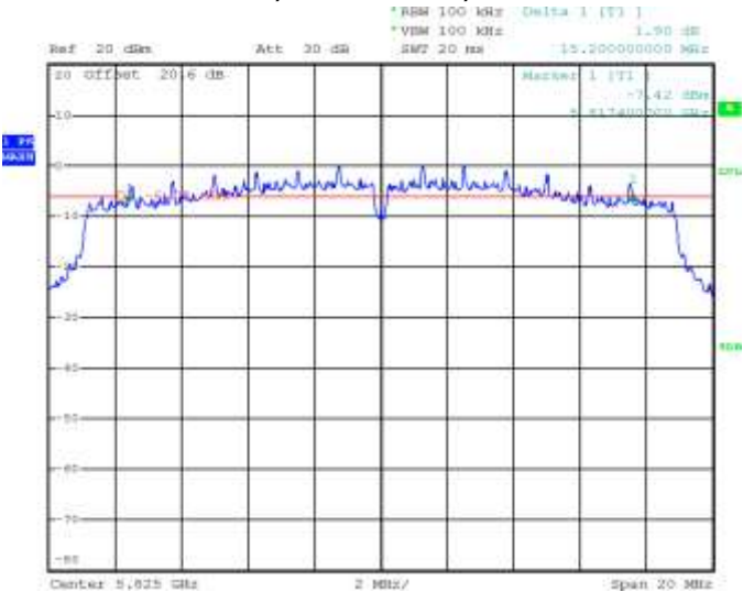
Figure 4-9: 6 dB Bandwidth 802.11n, Channel 165, MCS 0
