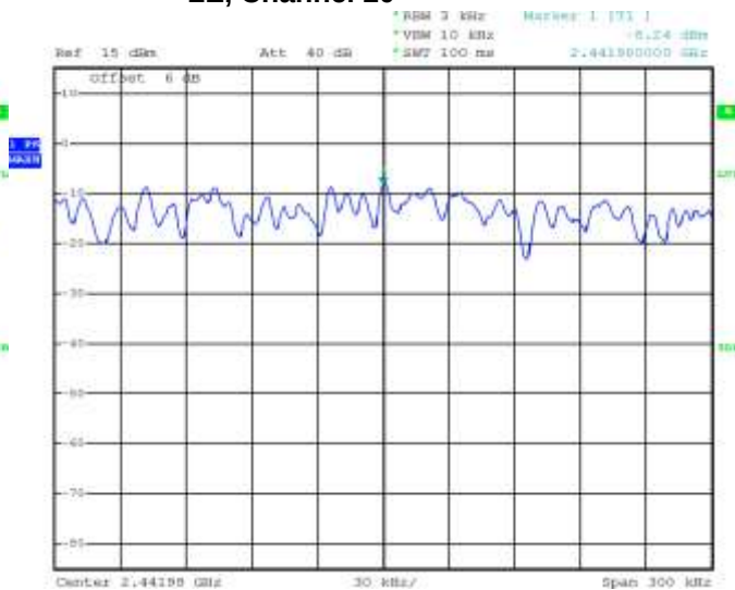
Figure 2-65: Peak Power Spectral Density LE, Channel 20
