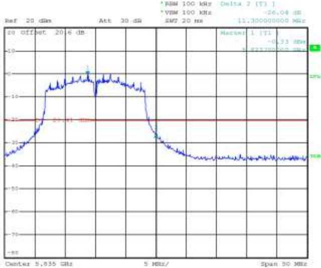
Figure 4-15: Band Edge Compliance 802.11a, Channel 165, 6 Mbps
