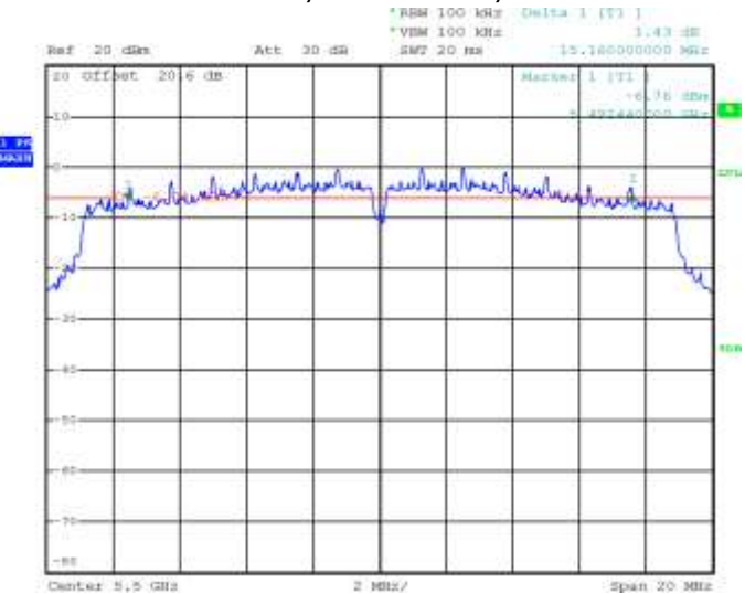
Figure 4-8: 6 dB Bandwidth 802.11n, Channel 100, MCS 0
