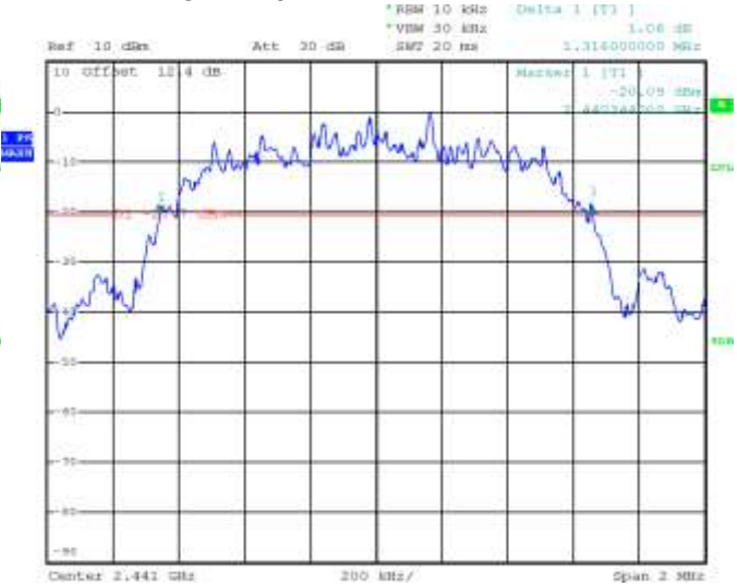
Figure 2-5: 20 dB Bandwidth Single freq., Static PBRS, 2-DH5
