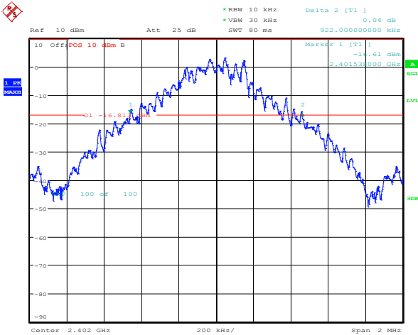
Figure 3-1: 20 dB Bandwidth Single freq., Static PBRS, DH5
