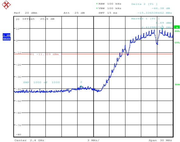
Figure 4-43: Band Edge Compliance 802.11b, Channel 1, 1 Mbps
