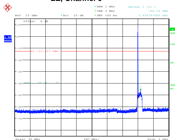
Figure 3-58: Spurious Conducted RF Emissions LE, Channel 0
