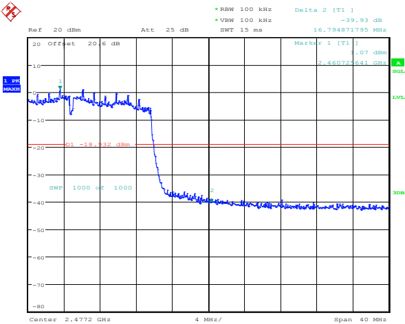
Figure 4-15: Band Edge Compliance 802.11n, Channel 11, MCS 0
