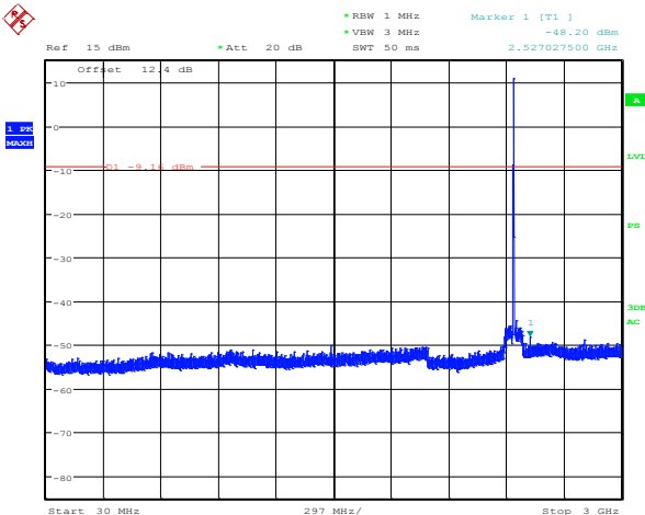
Figure 3-39: Spurious RF Conducted Emissions Single Freq., Static PBRS, DH5
