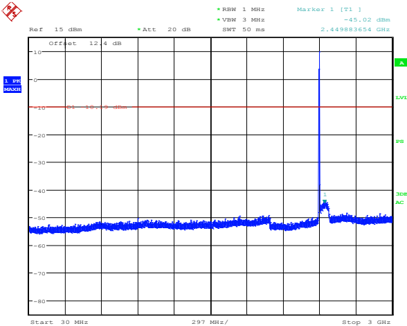
Figure 3-38: Spurious RF Conducted Emissions Single Freq., Static PBRS, DH5,
