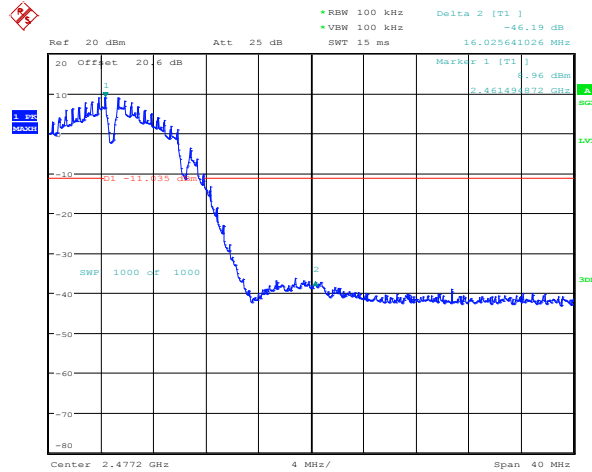
Figure 4-11: Band Edge Compliance 802.11b, Channel 11, 1 Mbps
