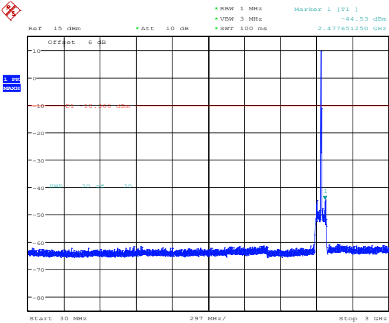
Figure 3-59 : Spurious Conducted RF Emissions LE, Channel 20
