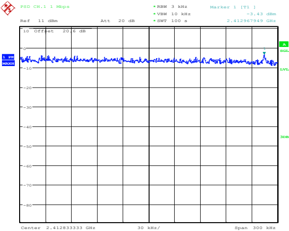
Figure 4-49: Peak Power Spectral Density 802.11b, Channel 1, 1 Mbps
