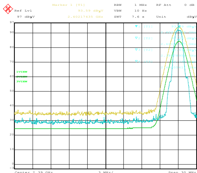
Figure 2-5: Band-Edge Compliance of RF Rad. Emissions. Bluetooth, Single freq., Static PBRs, 2-DH5, Channel 0, Pol: V
