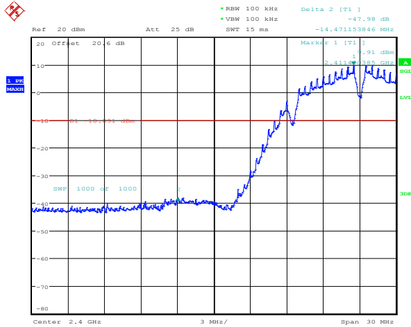
Figure 4-10: Band Edge Compliance 802.11b, Channel 1, 1 Mbps
