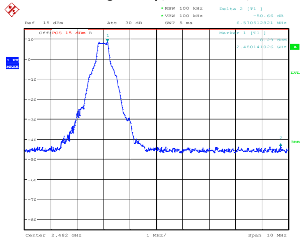
Figure 3-27: Band Edge Compliance Single Freq., Static PBRs, DH5
