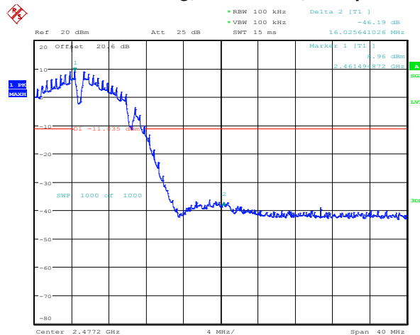
Figure 4-13: Band Edge Compliance 802.11g, Channel 11, 6 Mbps
