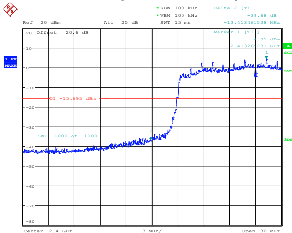
Figure 4-12: Band Edge Compliance 802.11g, Channel 1, 6 Mbps
