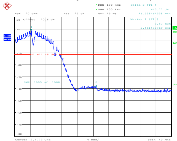
Figure 4-46: Band Edge Compliance 802.11g, Channel 11, 6 Mbps
