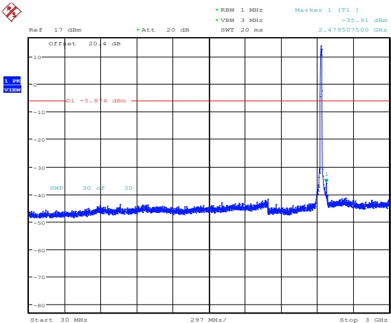
Figure 4-60: Spurious Conducted RF Emissions 802.11g, Channel 1, 6 Mbps
