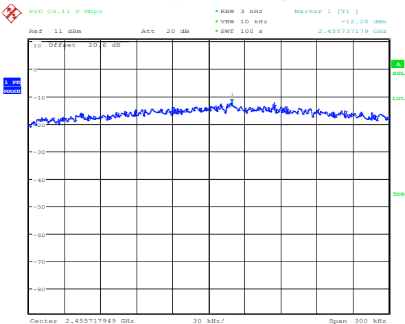
Figure 4-24: Peak Power Spectral Density 802.11n, Channel 11, MCS 0
