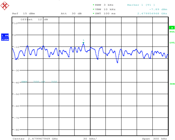
Figure 3-57: Peak Power Spectral Density LE, Channel 39
