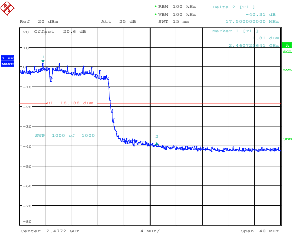
Figure 4-48: Band Edge Compliance 802.11n, Channel 11, MCS 0
