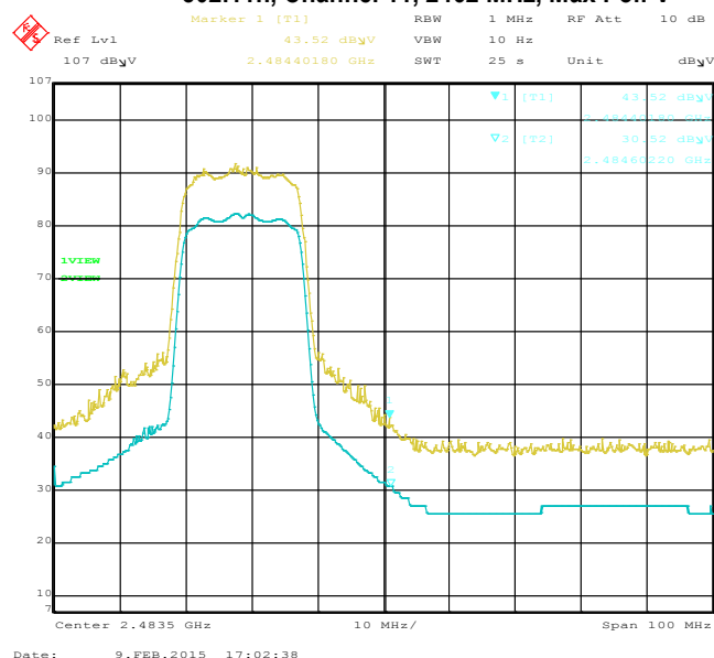
Figure 2-27: Band-Edge Compliance of RF Radiated Emission 802.11n, Channel 11, 2462 MHz, Max Pol: V
