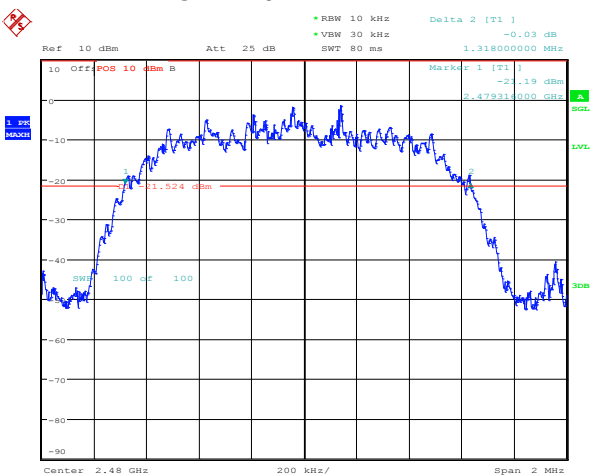
Figure 3-6: 20 dB Bandwidth Single freq., Static PBRS, 2-DH5
