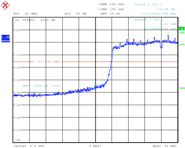
Figure 4-14: Band Edge Compliance 802.11n, Channel 1, MCS 0
