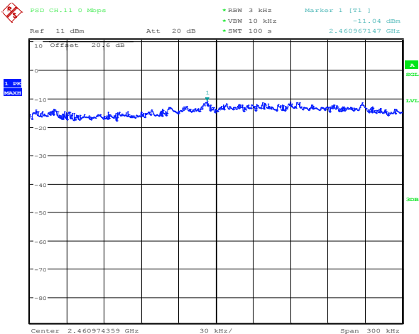
Figure 4-57: Peak Power Spectral Density 802.11n, Channel 11, MCS 0
