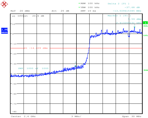
Figure 4-47: Band Edge Compliance 802.11n, Channel 1, MCS 0
