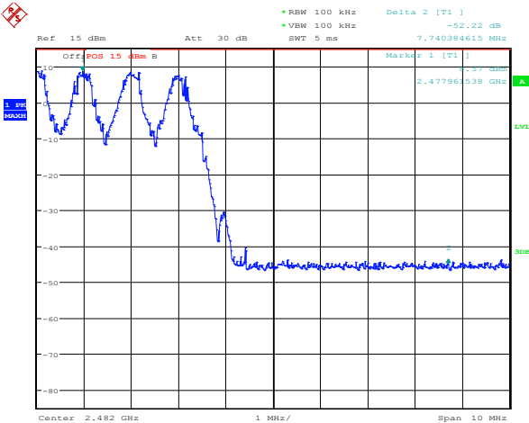
Figure 3-29: Band Edge Compliance Freq. Hopping, Static PBRS, DH5
