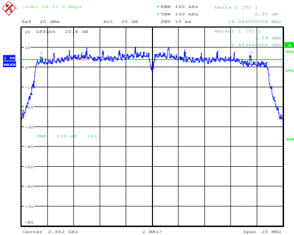
Figure 4-42: 6 dB Bandwidth 802.11n, Channel 11, MCS 0
