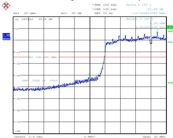
Figure 4-45: Band Edge Compliance 802.11g, Channel 1, 6 Mbps
