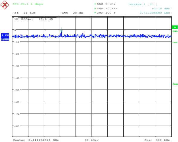
Figure 4-16: Peak Power Spectral Density 802.11b, Channel 1, 1 Mbps
