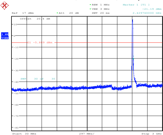
Figure 4-58 : Spurious Conducted RF Emissions 802.11b, Channel 6, 1 Mbps
