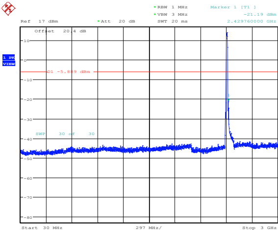
Figure 4-26 : Spurious Conducted RF Emissions 802.11b, Channel 6, 1 Mbps
