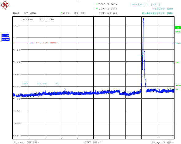
Figure 4-61: Spurious Conducted RF Emissions 802.11g, Channel 6, 6 Mbps
