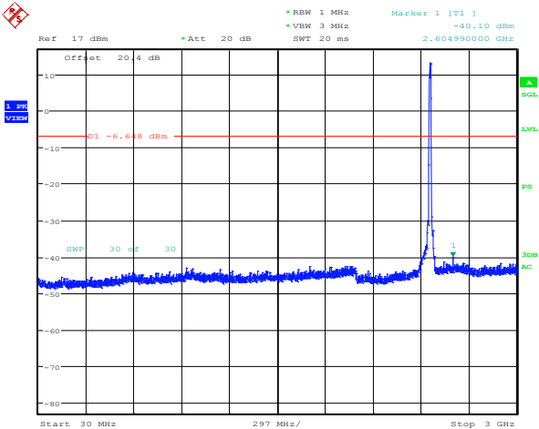
Figure 4-31: Spurious Conducted RF Emissions 802.11n, Channel 1, MCS 0
