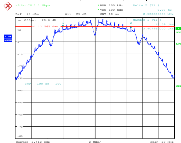
Figure 4-34: 6 dB Bandwidth 802.11b, Channel 1, 1 Mbps
