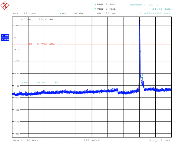
Figure 4-57: Spurious Conducted RF Emissions 802.11b, Channel 1, 1 Mbps
