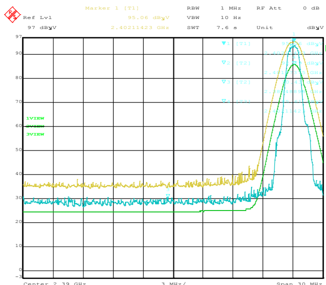
Figure 2-6: Band-Edge Compliance of RF Rad. Emissions. Bluetooth, Single freq., Static PBRs, 2-DH5, Channel 0, Pol: H
