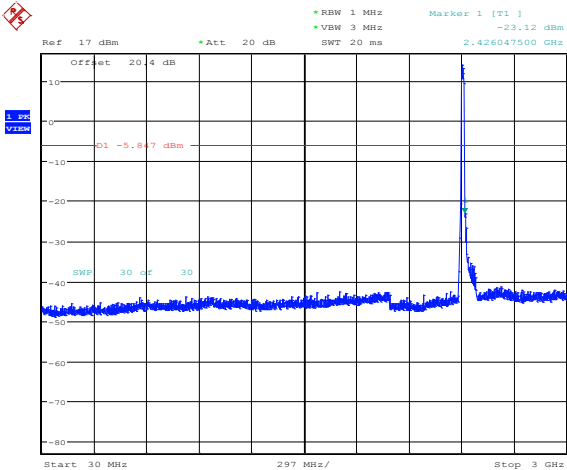
Figure 4-27: Spurious Conducted RF Emissions 802.11b, Channel 11, 1 Mbps
