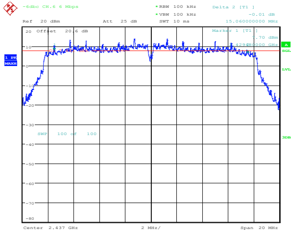
Figure 4-38: 6 dB Bandwidth 802.11g, Channel 6, 6 Mbps
