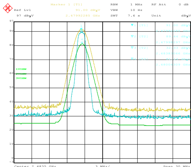
Figure 2-7: Band-Edge Compliance of RF Rad. Emissions. Bluetooth, Single freq., Static PBRs, 2-DH5, Channel 78, Pol: V
