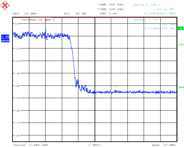
Figure 3-33: Band Edge Compliance Freq. Hopping, Static PBRS, 2-DH5
