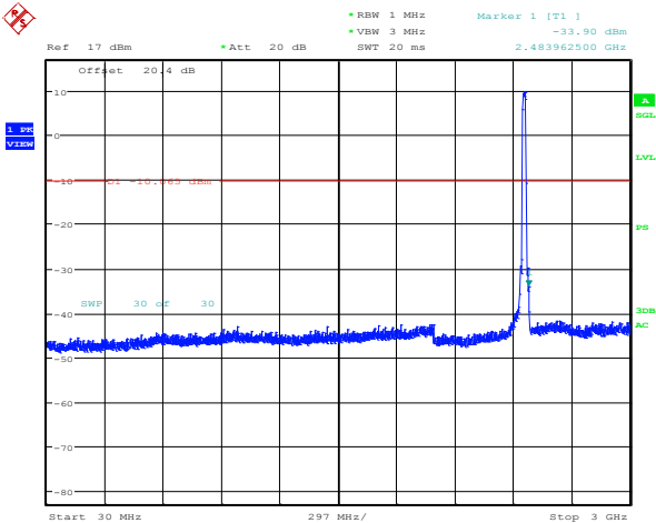
Figure 4-33: Spurious Conducted RF Emissions 802.11n, Channel 11, MCS 0
