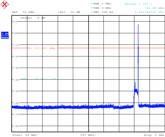
Figure 3-60: Spurious Conducted RF Emissions LE, Channel 39
