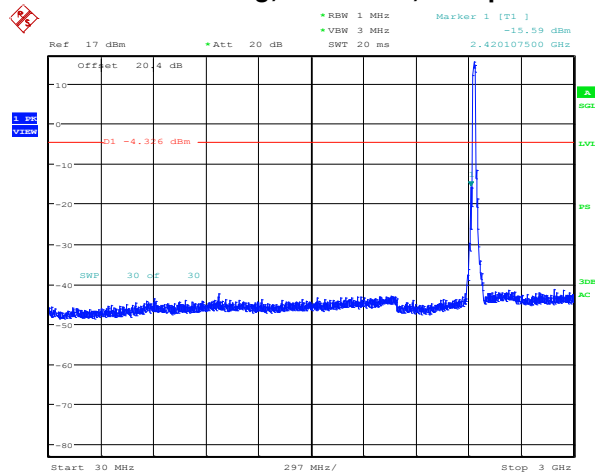
Figure 4-29: Spurious Conducted RF Emissions 802.11g, Channel 6, 6 Mbps
