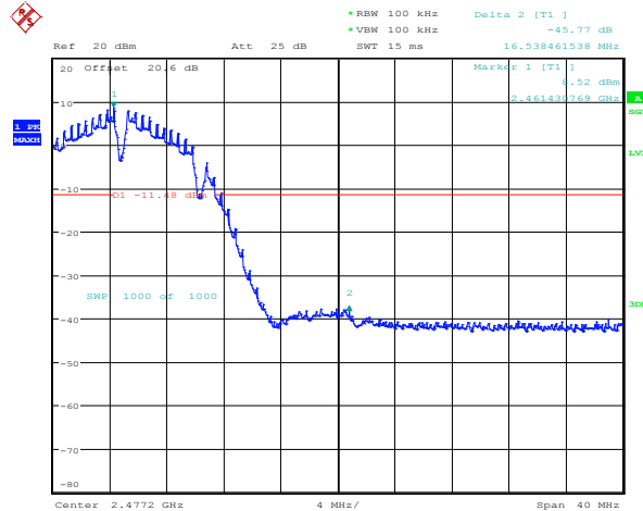
Figure 4-44: Band Edge Compliance 802.11b, Channel 11, 1 Mbps
