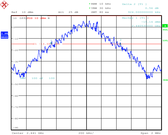
Figure 3-2: 20 dB Bandwidth Single freq., Static PBRS, DH5
