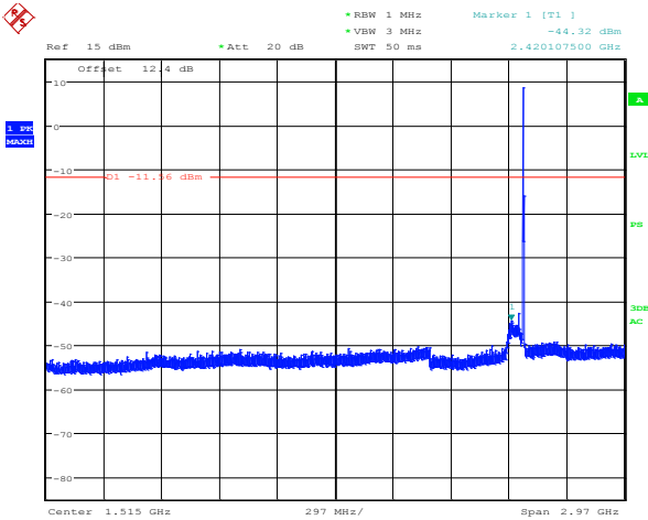
Figure 3-40: Spurious RF Conducted Emissions Single Freq., Static PBRS, DH5
