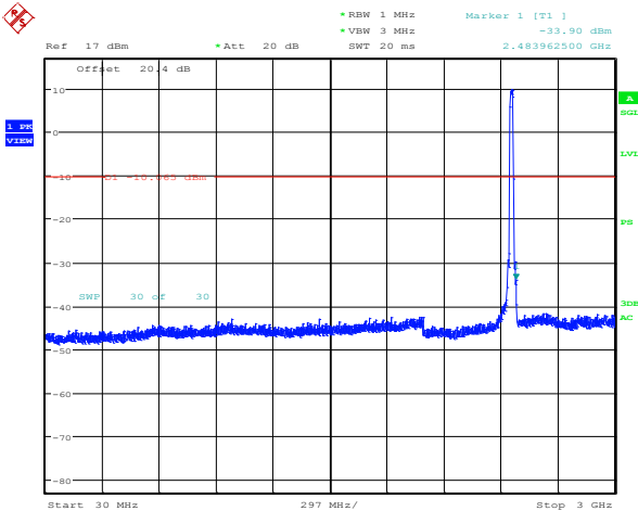
Figure 4-65: Spurious Conducted RF Emissions 802.11n, Channel 11, MCS 0
