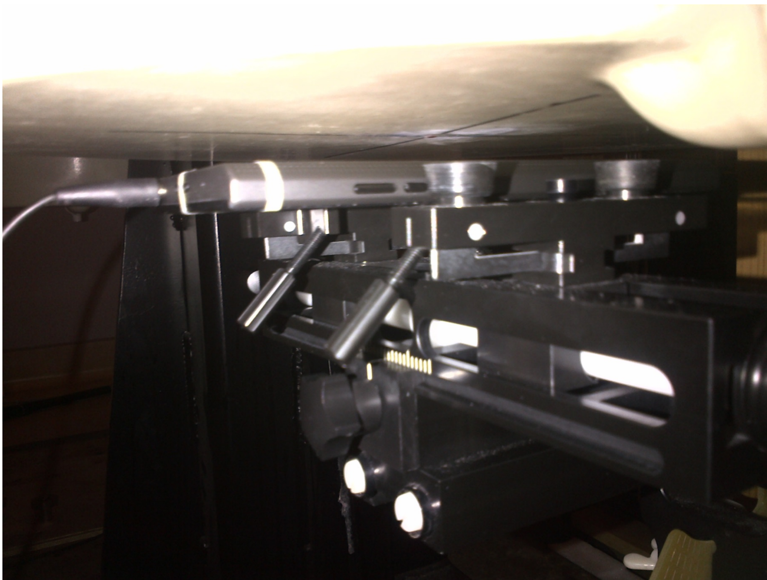
Figure E12. Hotspot configuration (No Holster, Headset, back side 10mm away)
