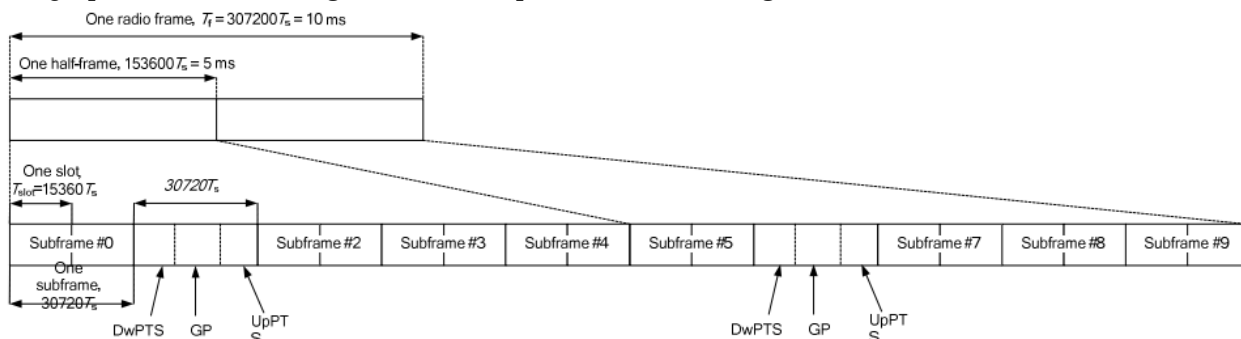
Figure 1: Frame structure type 2 (for 5ms switch-point periodicity)
