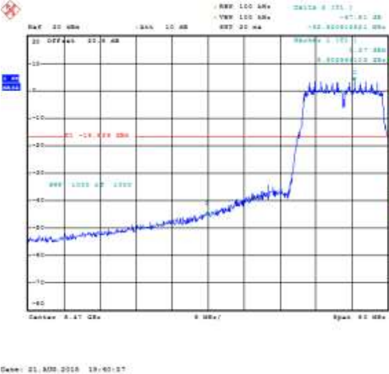
Figure 8-39: Band Edge Compliance Secondary, 802.11ac, Channel 100, MCS0 Mbps
