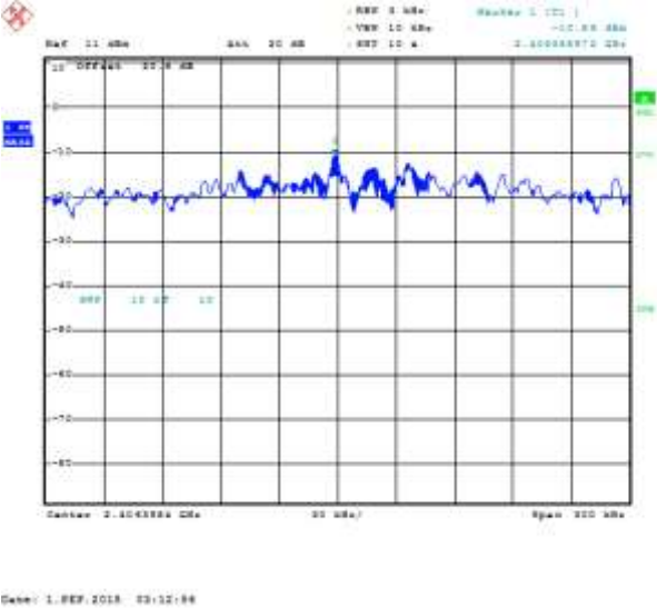
Figure 6-53: Peak Power Spectral Density MIMO Secondary, 802.11b, Channel 6, 1 Mbps
