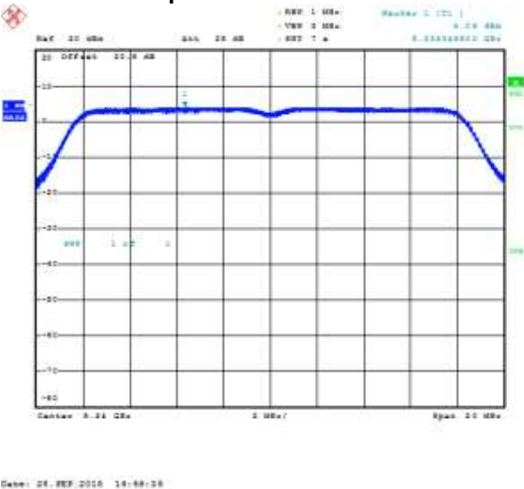
Figure 7-85: Peak Power Spectral Density MIMO Secondary, 802.11a, Channel 48, 6 Mbps
