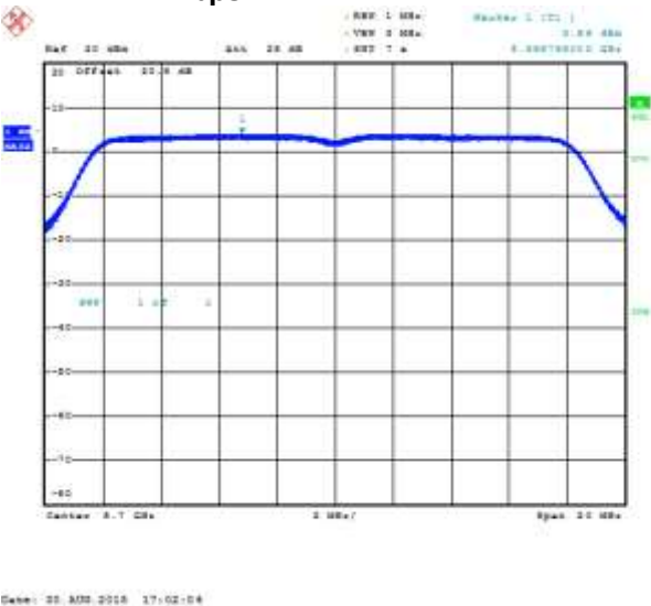
Figure 7-82: Peak Power Spectral Density MIMO Primary, 802.11a, Channel 140, 6 Mbps
