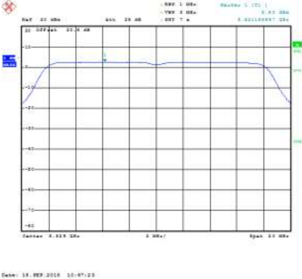
Figure 7-77: Peak Power Spectral Density SISO Secondary, 802.11a, Channel 165, 6 Mbps
