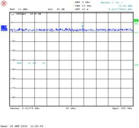
Figure 6-34: Peak Power Spectral Density SISO Secondary, 802.11b, Channel 1, 1 Mbps
