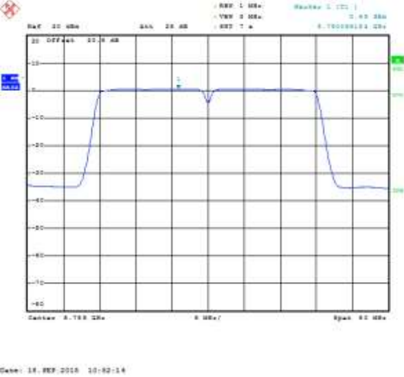
Figure 8-82: Peak Power Spectral Density SISO Primary, 802.11ac, Channel 151, MCS0 Mbps
