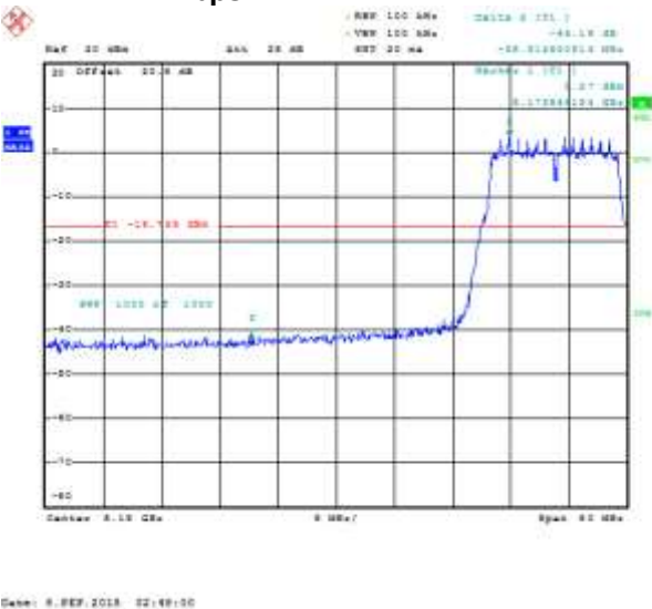
Figure 8-31: Band Edge Compliance Primary, 802.11ac, Channel 36, MCS0 Mbps
