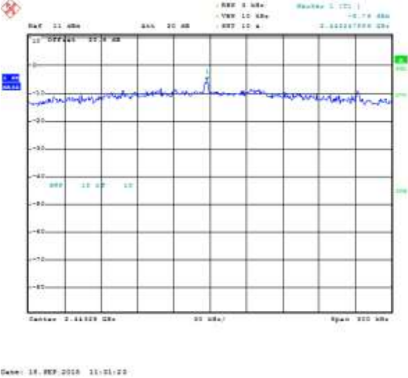
Figure 6-39: Peak Power Spectral Density SISO Secondary, 802.11g, Channel 11, 6 Mbps
