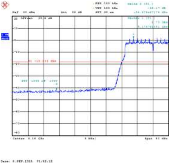
Figure 7-50: Band Edge Compliance Secondary, 802.11n, Channel 36, 6 Mbps
