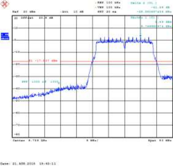
Figure 8-41: Band Edge Compliance Secondary, 802.11ac, Channel 149, MCS0 Mbps
