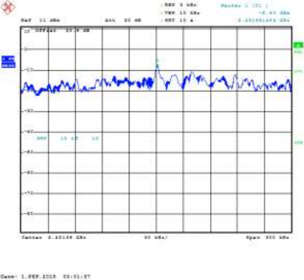
Figure 6-47: Peak Power Spectral Density MIMO Primary, 802.11g, Channel 6, 6 Mbps
