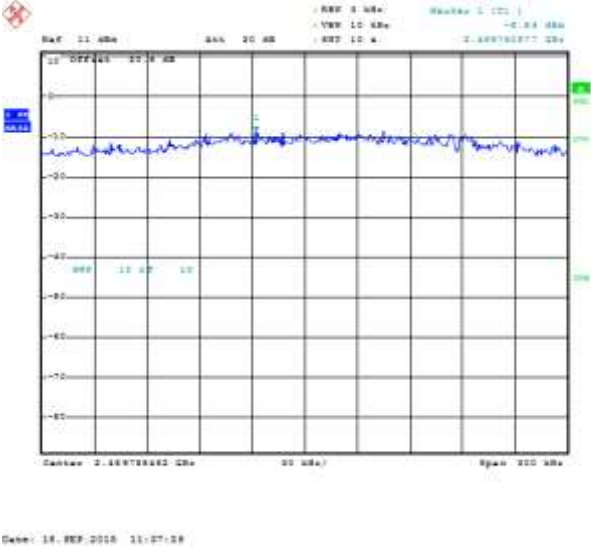
Figure 6-42: Peak Power Spectral Density SISO Secondary, 802.11n, Channel 11, MCS 0
