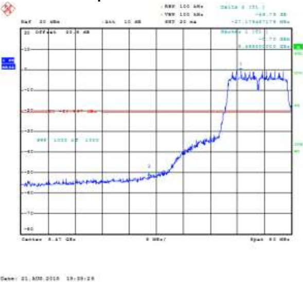
Figure 8-33: Band Edge Compliance Primary, 802.11ac, Channel 100, MCS0 Mbps
