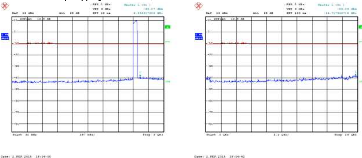
Figure 5-41: Spurious RF Conducted Emissions Freq. Hopping, Static PBRs, DH5
