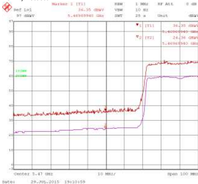
Figure 4-39: Band-Edge Compliance of RF Radiated Emission 802.11ac, Secondary, Ch. 106, 5530 MHz, Centre of Band-Edge: 5470 MHz Pol: V, Detector: PK
