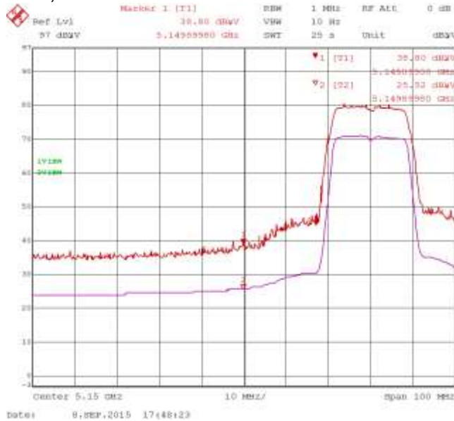
Figure 3-23: Band-Edge Compliance of RF Radiated Emission 802.11n, Secondary, Ch. 36, 5180 MHz, Centre of Band-Edge: 5150 MHz Pol: V, Detector: PK
