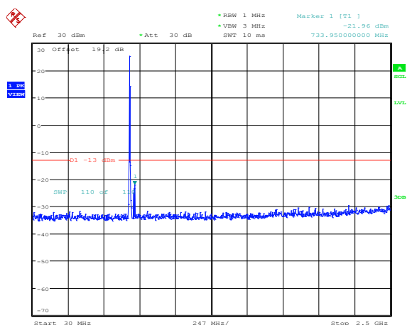
Figure 3-7a: Band 12, Spurious Conducted Emissions, Low channel, 5MHz BW (RB= 1)
