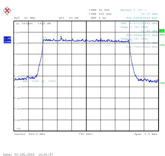
Figure 4-30a: Occupied Bandwidth, Band 5 High Channel, 5MHz BW, RB=25
