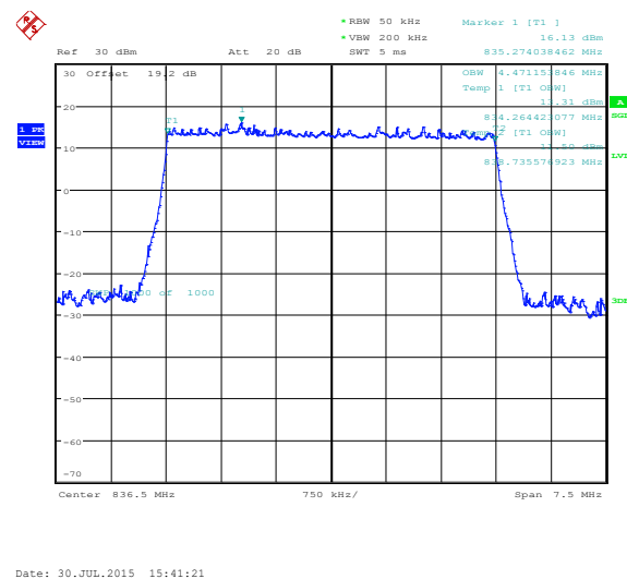
Figure 4-29a: Occupied Bandwidth, Band 5 Middle Channel, 5MHz BW, RB=25
