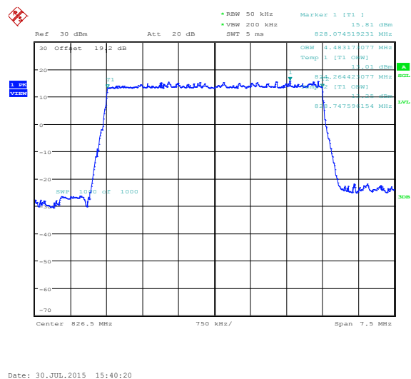
Figure 4-28a: Occupied Bandwidth, Band 5 Low Channel, 5MHz BW, RB=25
