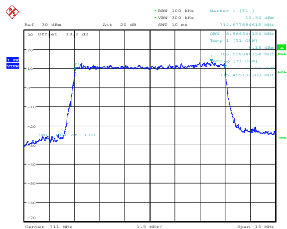
Figure 6-15a: Occupied Bandwidth, Band 17 High Channel, 10MHz BW, RB=50
