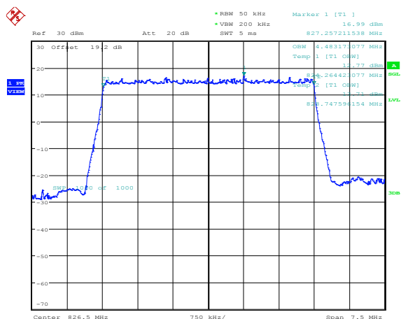
Figure 4-25a: Occupied Bandwidth, Band 5 Low Channel, 5MHz BW, RB=25
