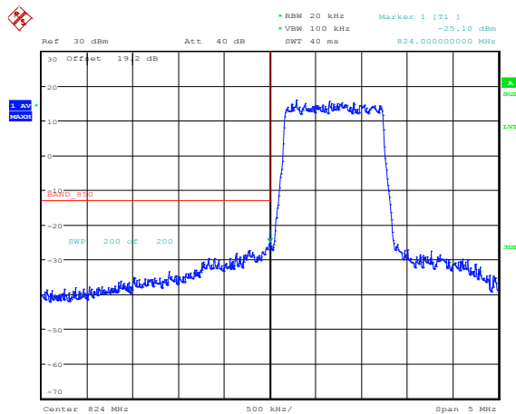
Figure 4-56a: Band 5 Low Channel Mask, 1.4MHz BW, RB=6
