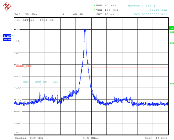
Figure 4-59a: Band 5 High Channel Mask, 10MHz BW, RB=1
