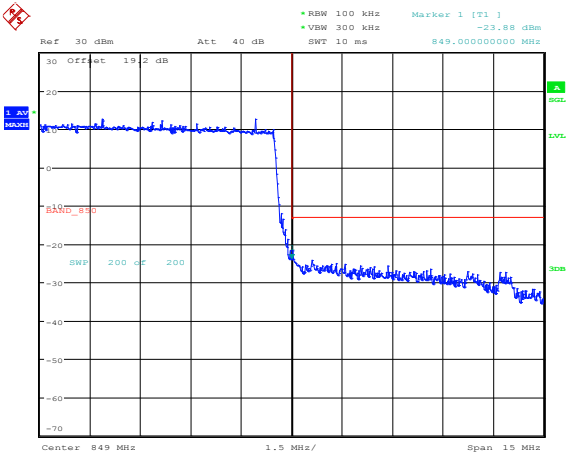
Figure 4-53a: Band 5 High Channel Mask, 10MHz BW, RB=50
