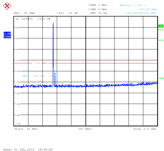
Figure 3-9a: Band 12, Spurious Conducted Emissions, Middle Channel, 5MHz BW (RB= 25)
