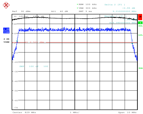
Figure 4-43a: -26 dBc Bandwidth, Band 5 Low Channel, 10MHz BW, RB=50
