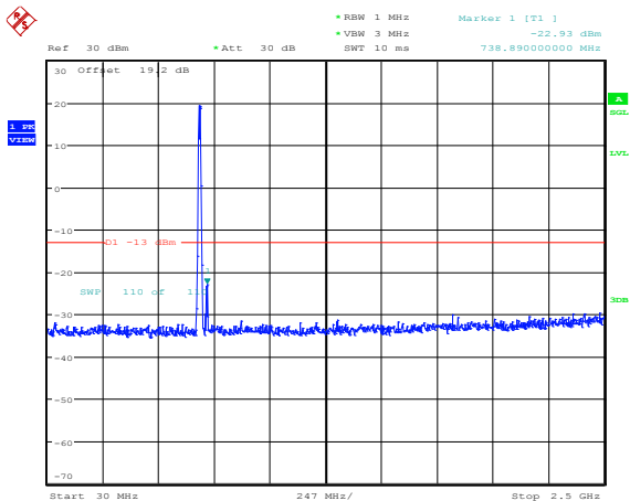
Figure 3-5a: Band 12, Spurious Conducted Emissions, High Channel, 10MHz BW (RB= 100)
