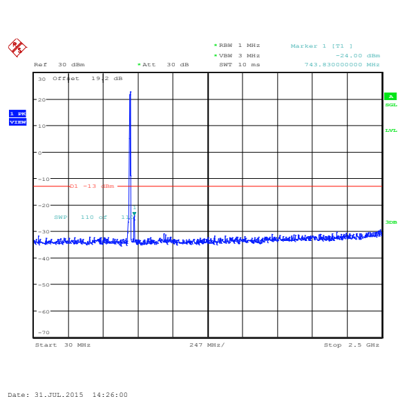
Figure 3-11a: Band 12, Spurious Conducted Emissions, High channel, 5MHz BW (RB= 50)
