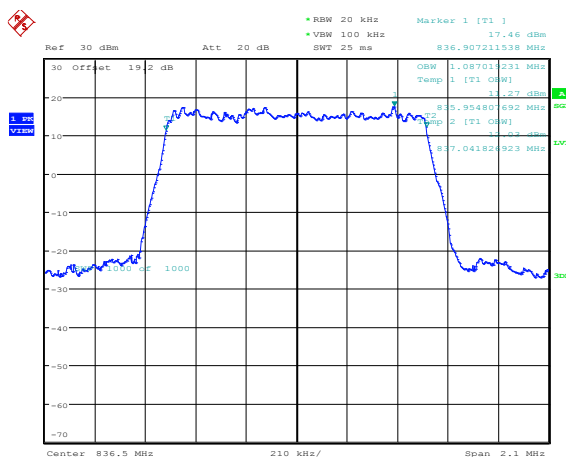
Figure 4-41a: Occupied Bandwidth, Band 5 Middle Channel, 1.4MHz BW, RB=6
