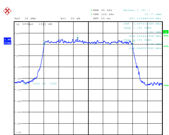
Figure 4-36a: Occupied Bandwidth, Band 5 High Channel, 3MHz BW, RB=15
