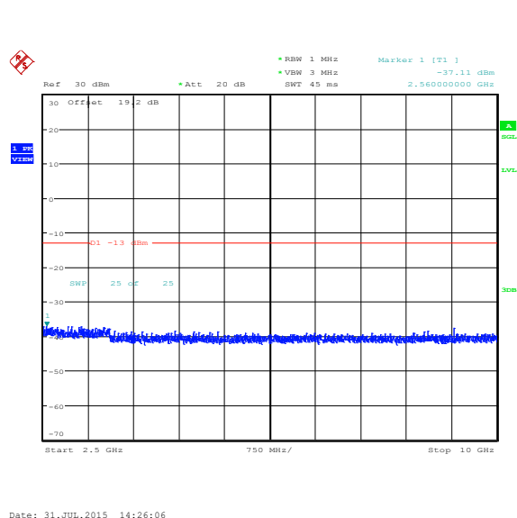
Figure 3-12a: Band 12, Spurious Conducted Emissions, High channel, 5MHz BW (RB= 50)
