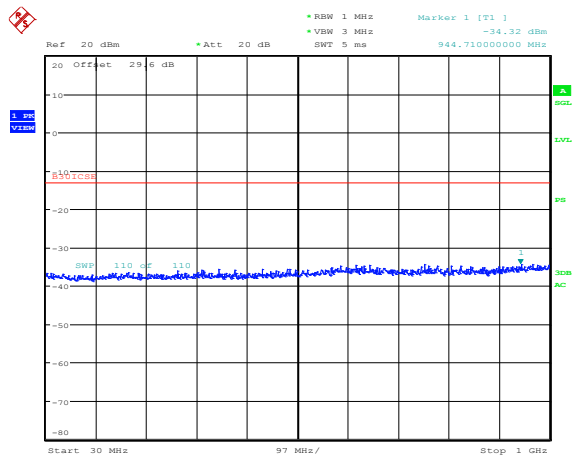
Figure 8-7a: Band 30, Spurious Conducted Emissions, Low channel, 5MHz BW (RB= 1)
