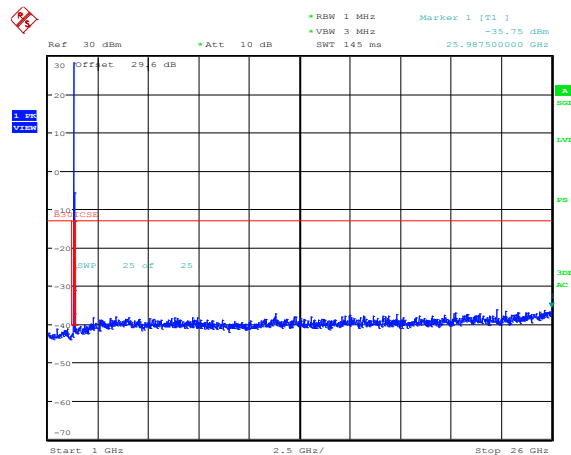
Figure 8-8a: Band 30, Spurious Conducted Emissions, Low channel, 5MHz BW (RB= 1)
