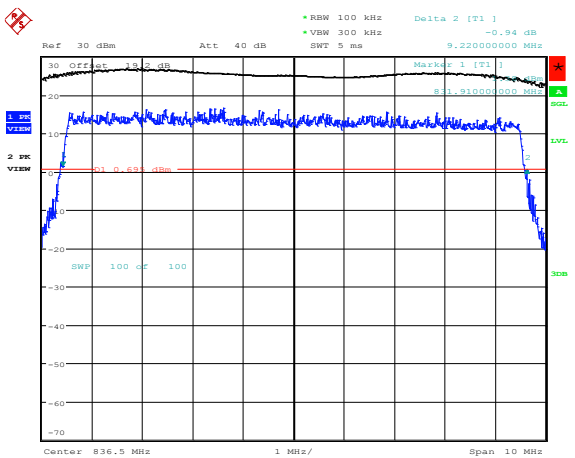
Figure 4-44a: -26 dBc Bandwidth, Band 5 Middle Channel, 10MHz BW, RB=50
