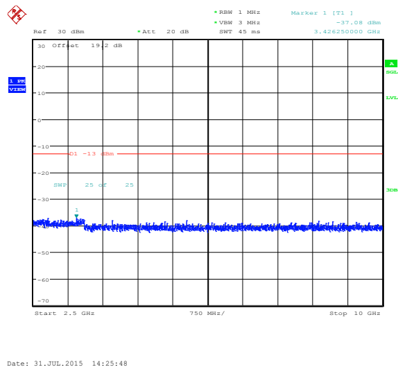
Figure 3-10a: Band 12, Spurious Conducted Emissions, Middle Channel, 5MHz BW (RB= 25)
