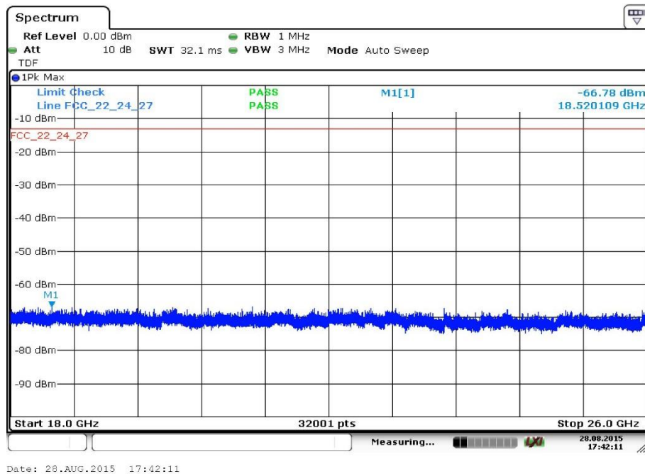
Plot 14: HSUPA Channel 9262 (18 GHz - 26 GHz)
