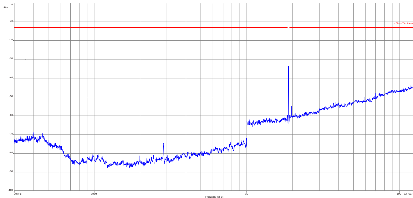
Plot 5: Voice Channel 9400 (30 MHz – 12.75 GHz)
