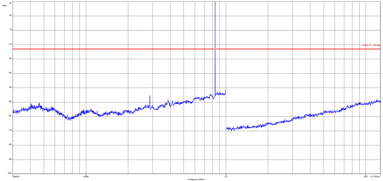
Plot 7: 8-PSK Channel 189 (30 MHz – 12.75 GHz)
