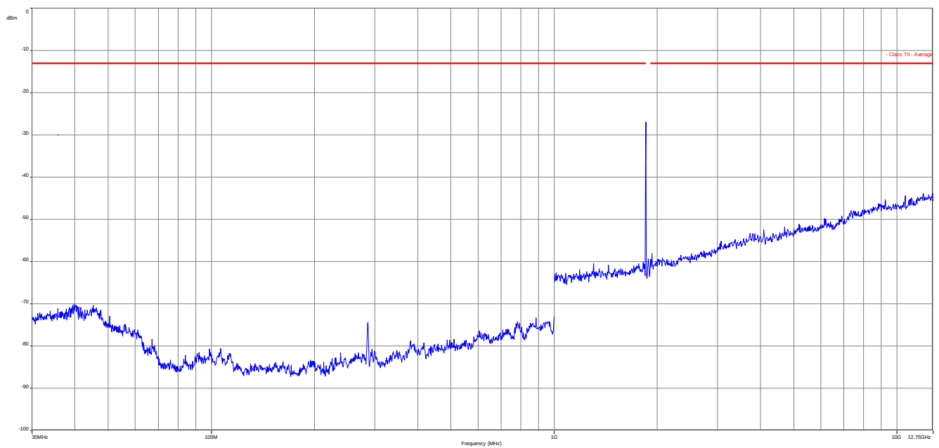
Plot 12: 8-PSK Channel 512 (30 MHz – 12.75 GHz)
