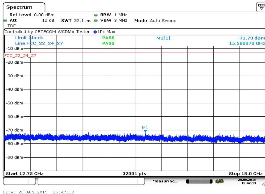
Plot 13: HSUPA Channel 9262 (12.75 GHz - 18 GHz)
