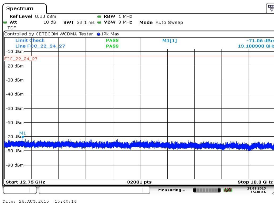
Plot 6: Voice Channel 9400 (12.75 GHz - 18 GHz)
