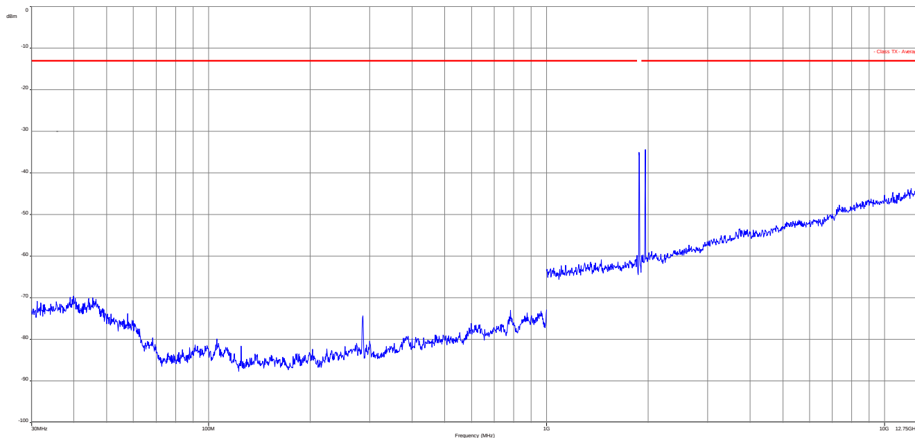
Plot 15: HSUPA Channel 9400 (30 MHz – 12.75 GHz)
