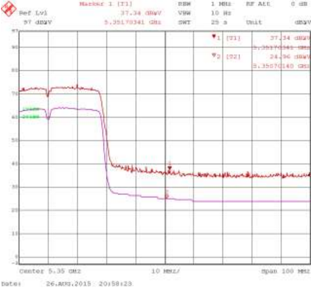
Figure 3-19 Band-Edge Compliance of RF Radiated Emission 802.11n, Primary, Ch. 62, 5310 MHz, Centre of Band-Edge: 5350 MHz
