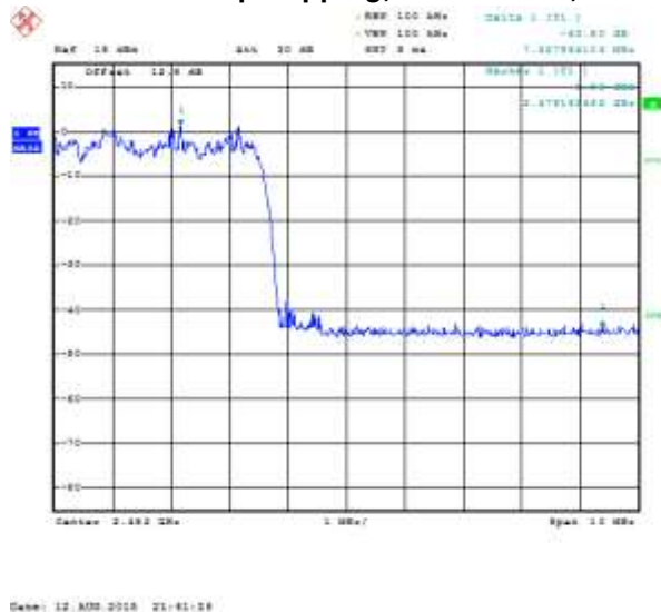
Figure 5-33: Band Edge Compliance Freq. Hopping, Static PBRS, 2-DH5
