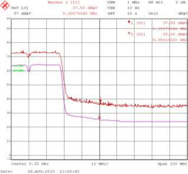
Figure 3-20: Band-Edge Compliance of RF Radiated Emission 802.11n, Primary, Ch. 62, 5310 MHz, Centre of Band-Edge: 5350 MHz
