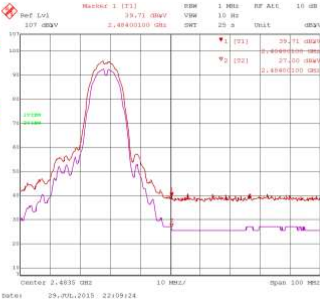
Figure 2-20: Band-Edge Compliance of RF Radiated Emission 802.11b, Channel 11, 2462 MHz, Max Pol: H, Detector: PK
