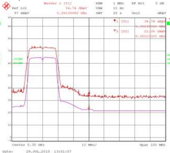
Figure 3-26: Band-Edge Compliance of RF Radiated Emission 802.11n, Secondary, Ch. 64, 5320 MHz, Centre of Band-Edge: 5350 MHz
