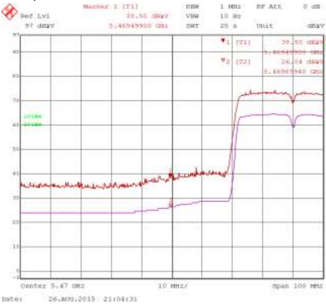
Figure 3-22: Band-Edge Compliance of RF Radiated Emission. 802.11n, Primary, Ch. 102, 5510 MHz, Centre of Band-Edge: 5470 MHz Pol: H, Detector: PK
