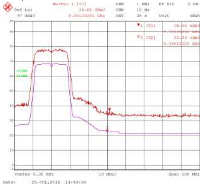
Figure 3-25: Band-Edge Compliance of RF Radiated Emission 802.11n, Secondary, Ch. 64, 5320 MHz, Centre of Band-Edge: 5350 MHz
