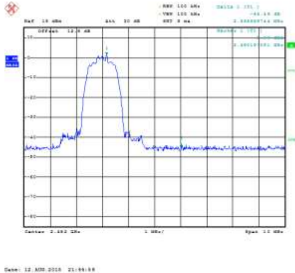
Figure 5-31: Band Edge Compliance Single Freq., Static PBRS, 2-DH5
