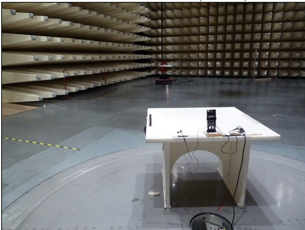
Photo 6: radiated emission 1-10GHz set 2 (slider closed)
