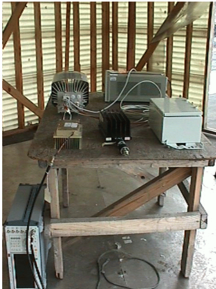
Photograph of Radiated Emissions Test Configuration
