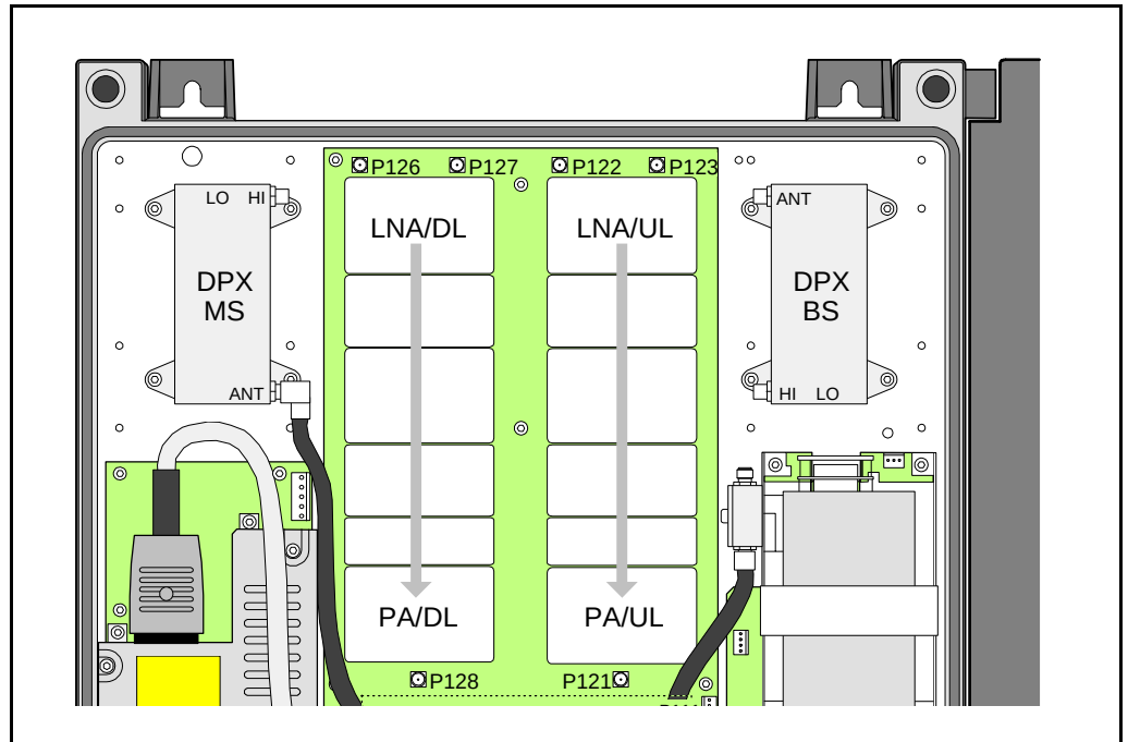
Figure 5-5. LNA, Low Noise Amplifiers
