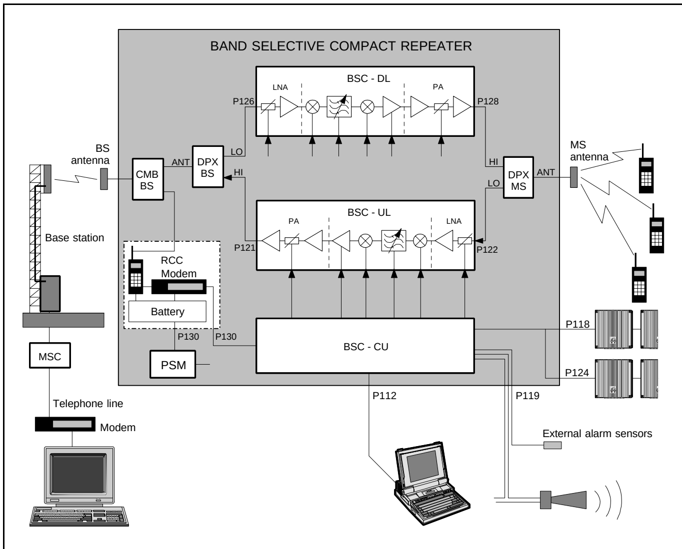
Figure 5-3. Block diagram
