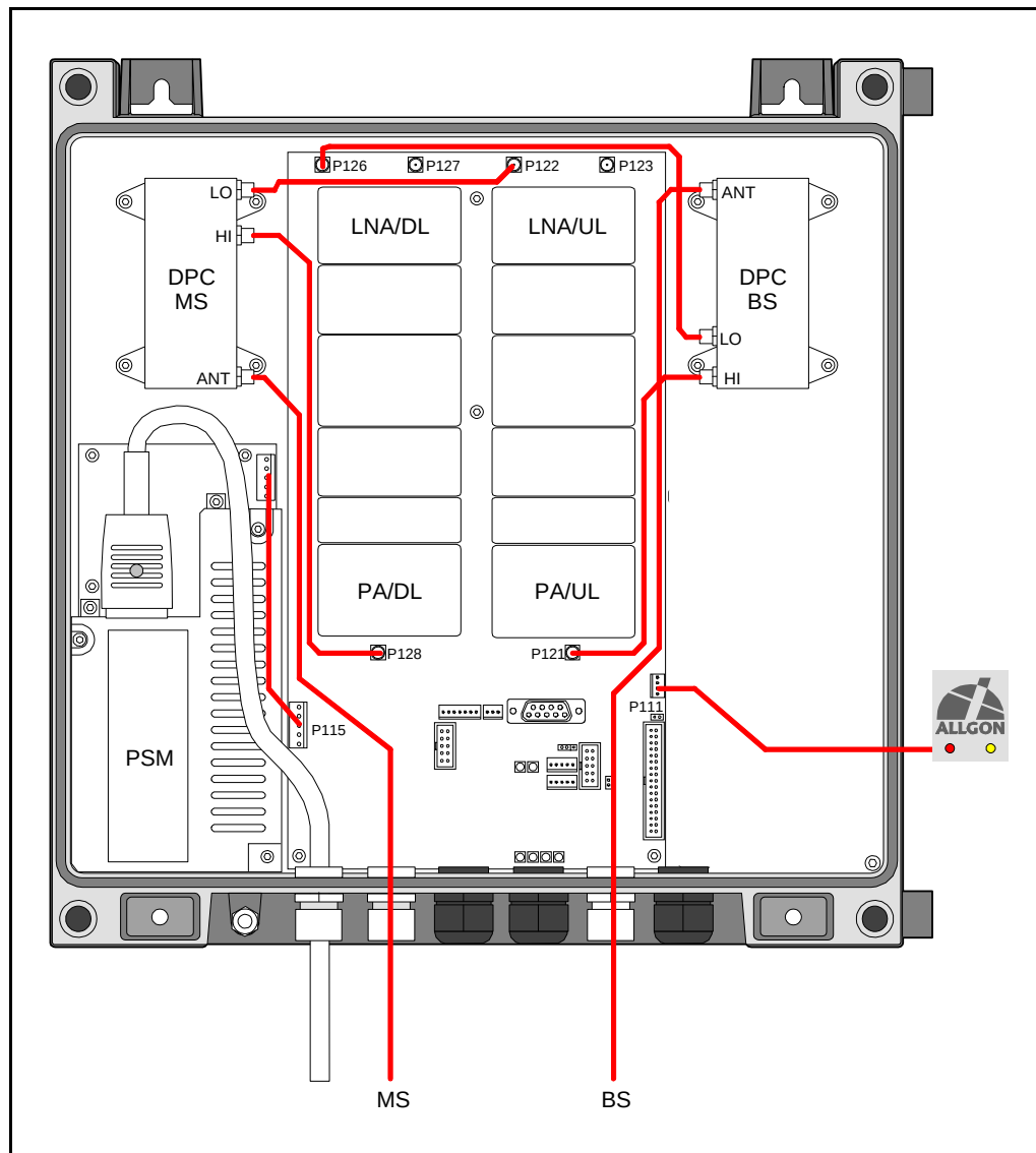
Figure 5-8. Cabling without RCC unit
