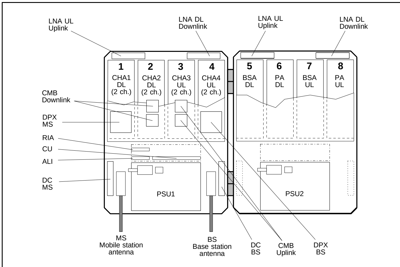
Figure 5-5. Combined repeater
