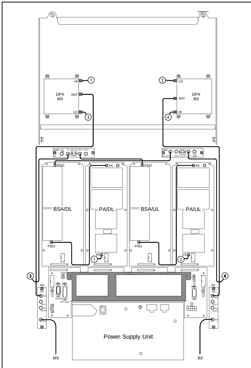
Figure 5-18. Cabling, band selective repeater
