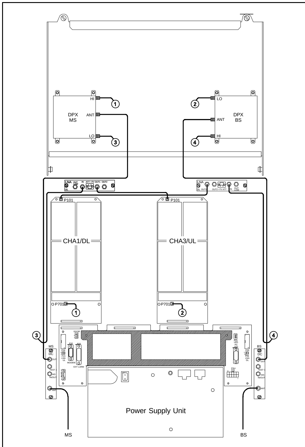
Figure 5-14. Cabling, GSM repeater - 2 ch.
