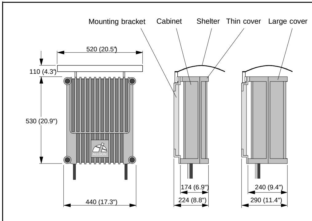
Figure 3-1. Repeater dimensions
