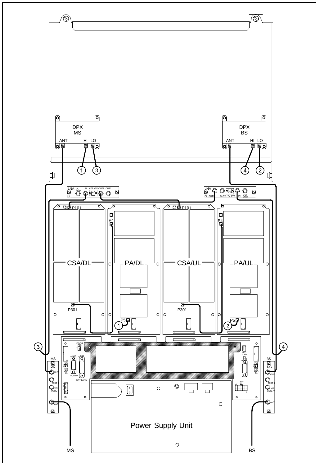
Figure 5-16. Cabling, CDMA repeater - 2 ch.
