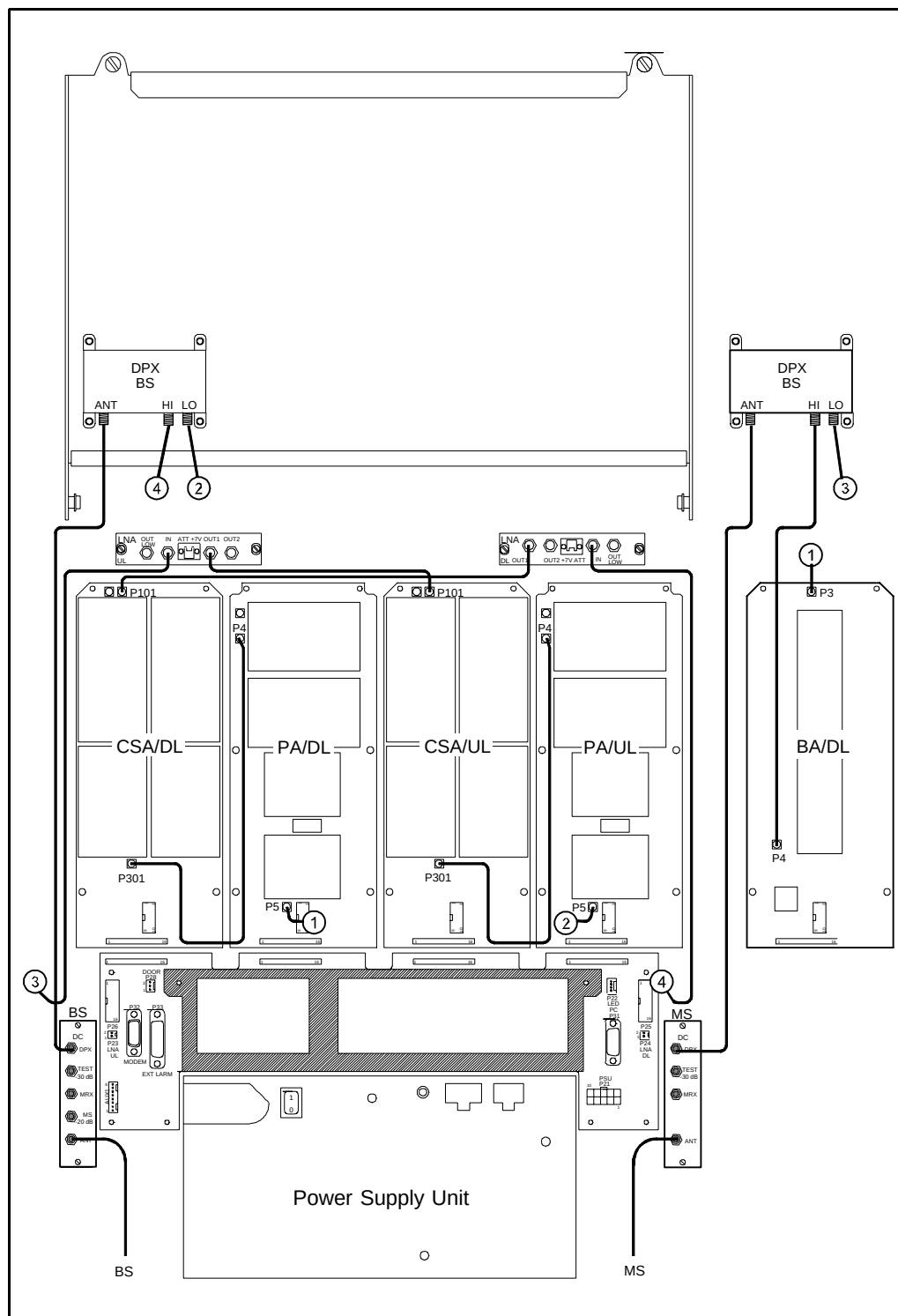
Figure 5-17. Cabling, high power CDMA repeater - 2 ch.
