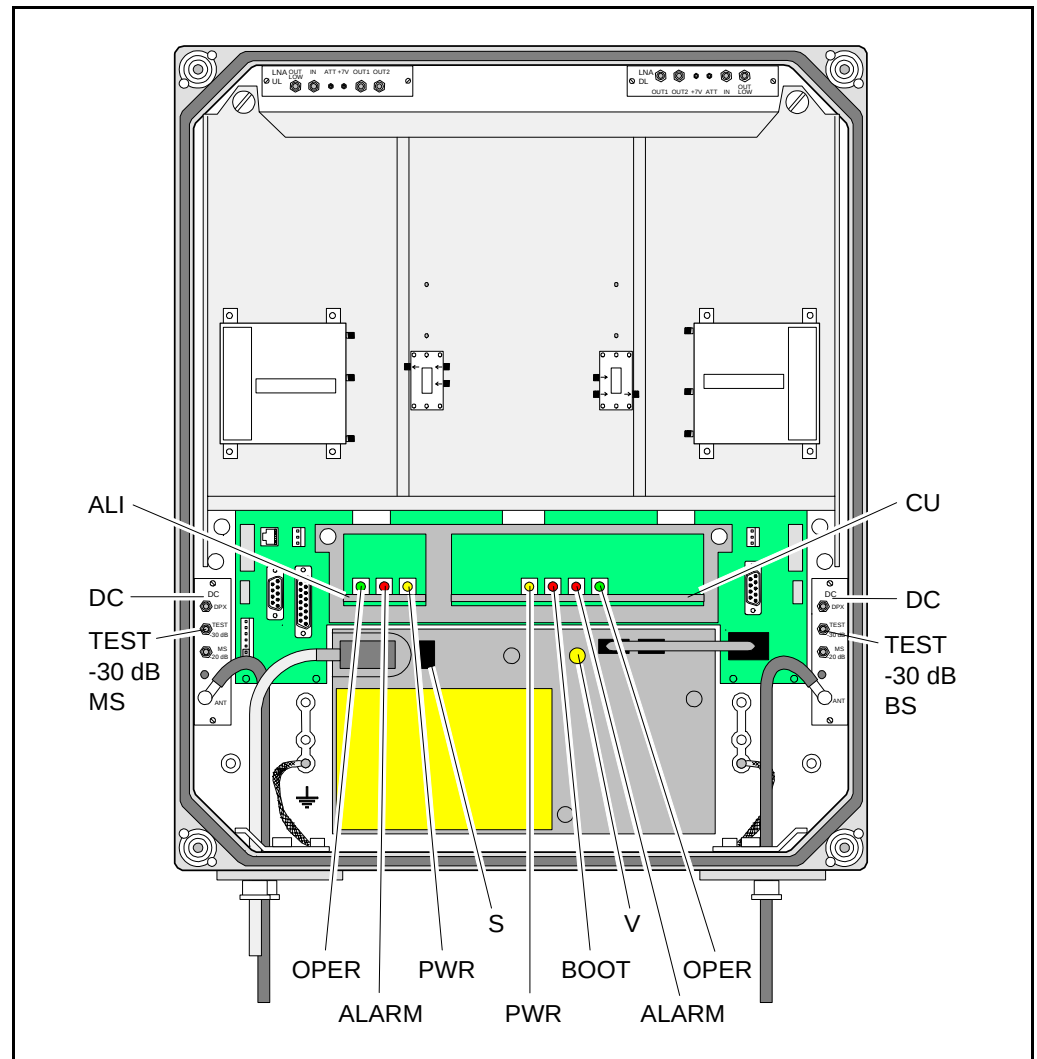
Figure 4-1. Indicators and mains switch
