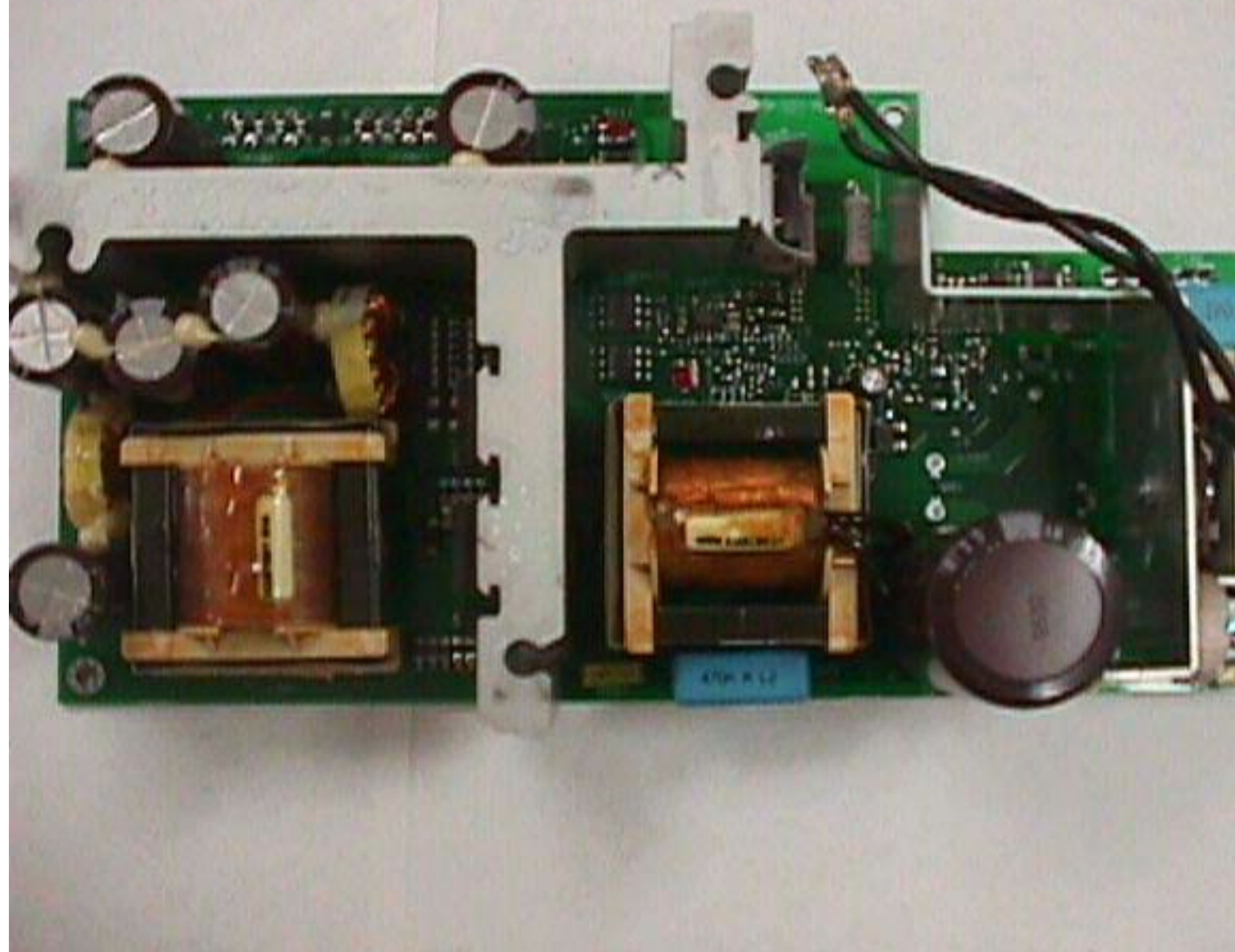
POWER SUPPLY PCB PARTS SIDE
