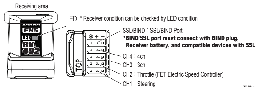
LED condition indicator
