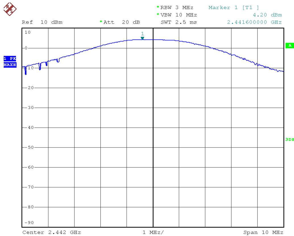
Figure 8: Peak output power - Middle channel
