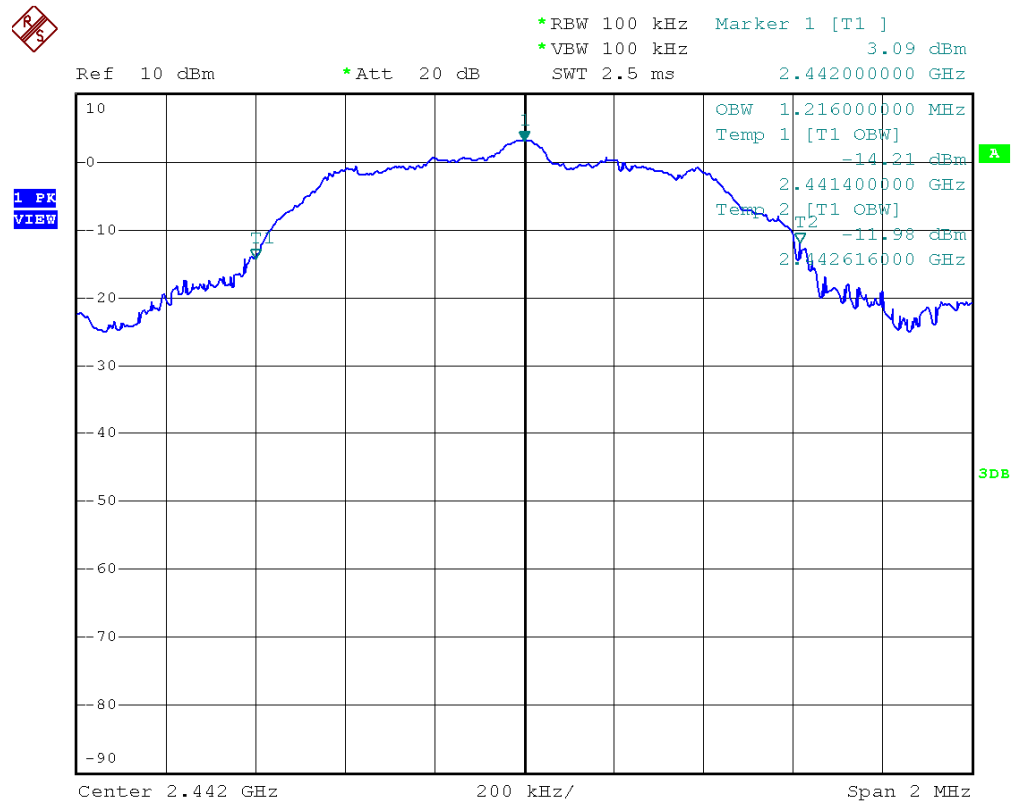
Figure 26- 99% Bandwidth measurement (fc=2442MHz)
