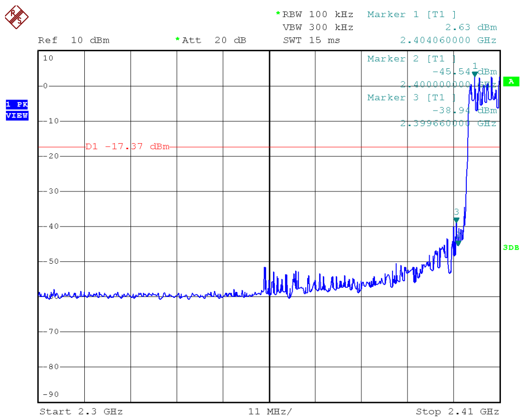
Figure 12: Band edge – Low frequency side with hopping
