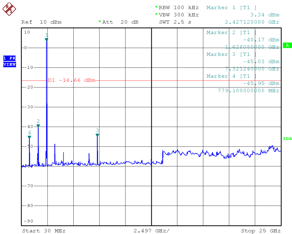
Figure 15 Conducted spurious emissions - Middle channel
