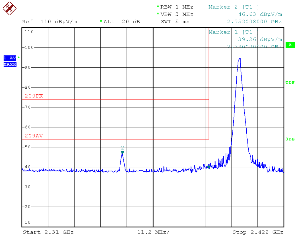
Figure 20 Band edge of radiated emission – Low frequency side without hopping Average measurement in vertical polarization
