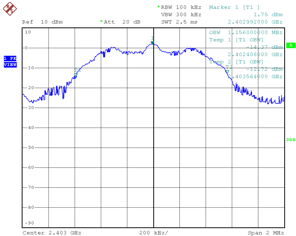
Figure 25- 99% Bandwidth measurement (fc=2403MHz)
