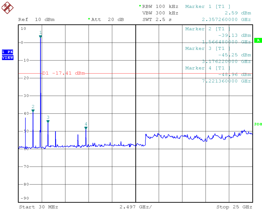
Figure 14 Conducted spurious emissions - Low channel
