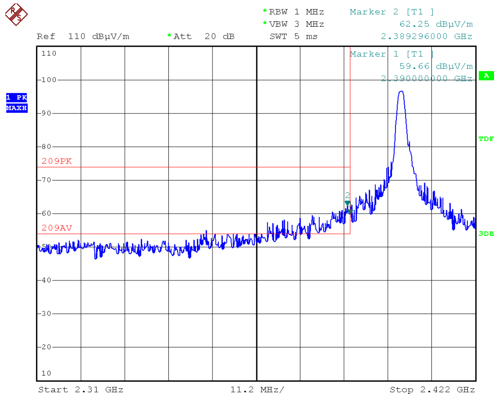
Figure 19 Band edge of radiated emission – Low frequency side with hopping Peak measurement in vertical polarization
