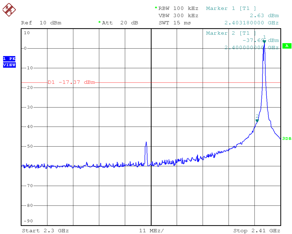
Figure 10: Band edge - Low frequency side without hopping
