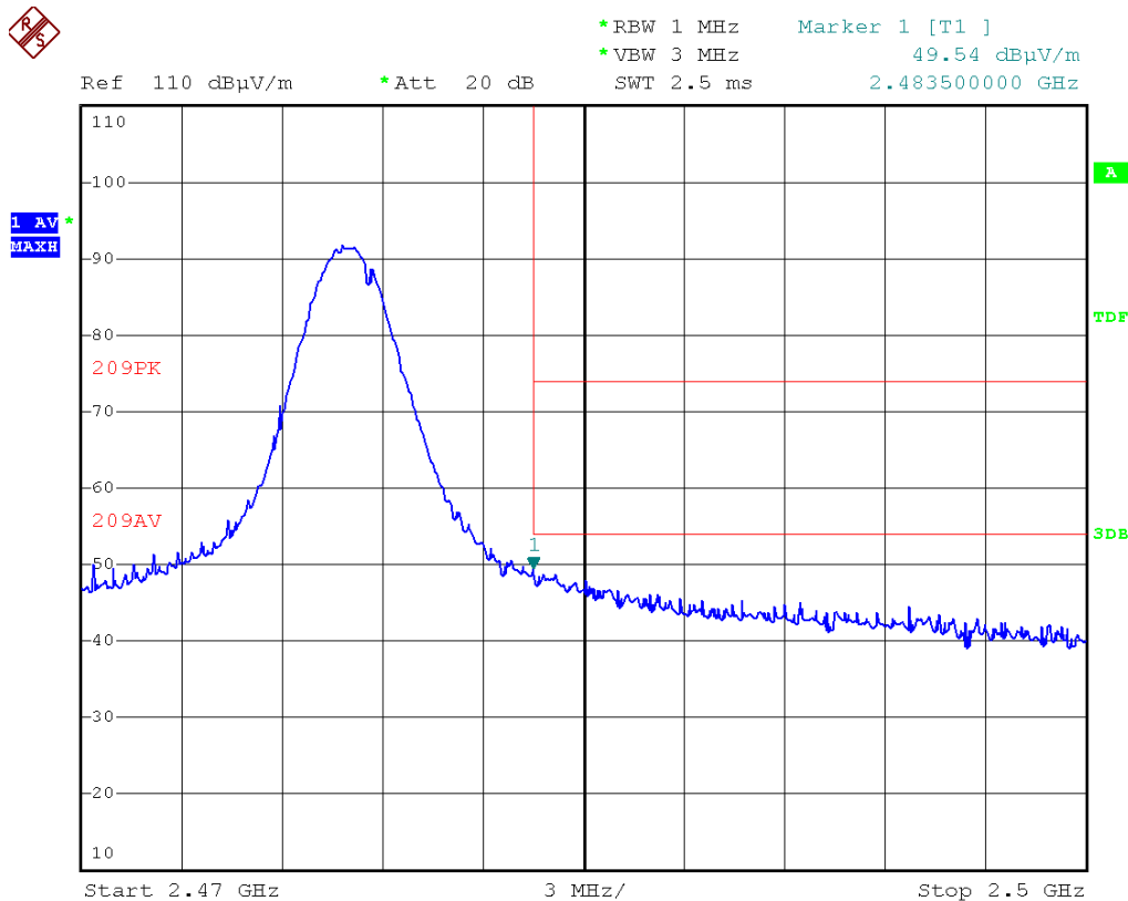
Figure 22 Band edge of radiated emission – High frequency side with hopping Average measurement in horizontal polarization
