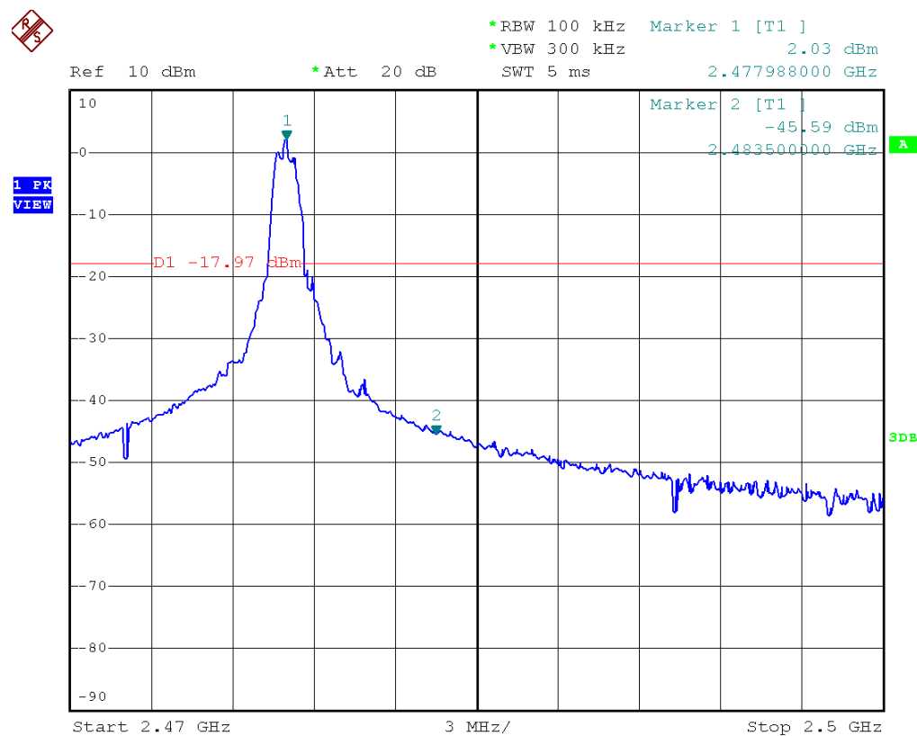
Figure 11: Band edge – High frequency side without hopping
