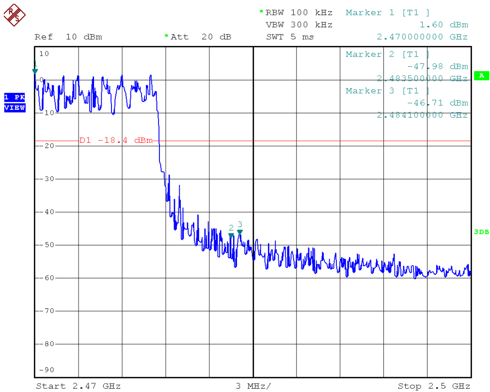
Figure 13: Band edge – High frequency side with hopping
