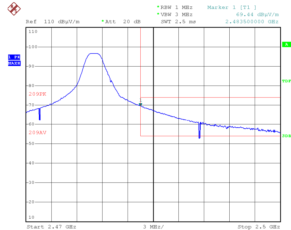
Figure 23 Band edge of radiated emission – High frequency side with hopping Peak measurement in vertical polarization
