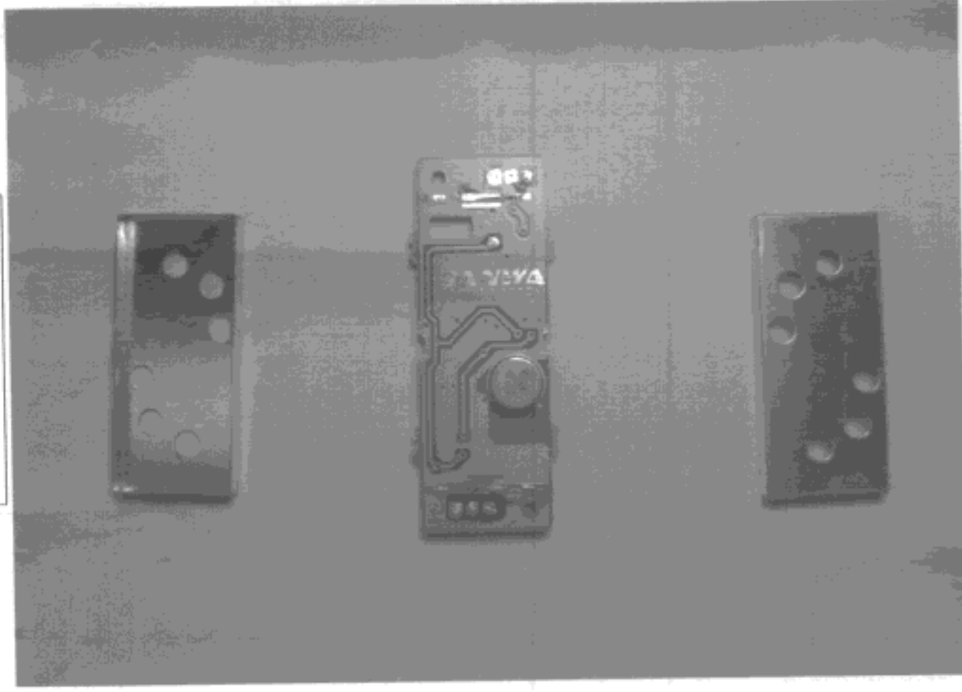
RF UNIT : CLOSE VIEW Reversed side view. Shielding covers are removed.
