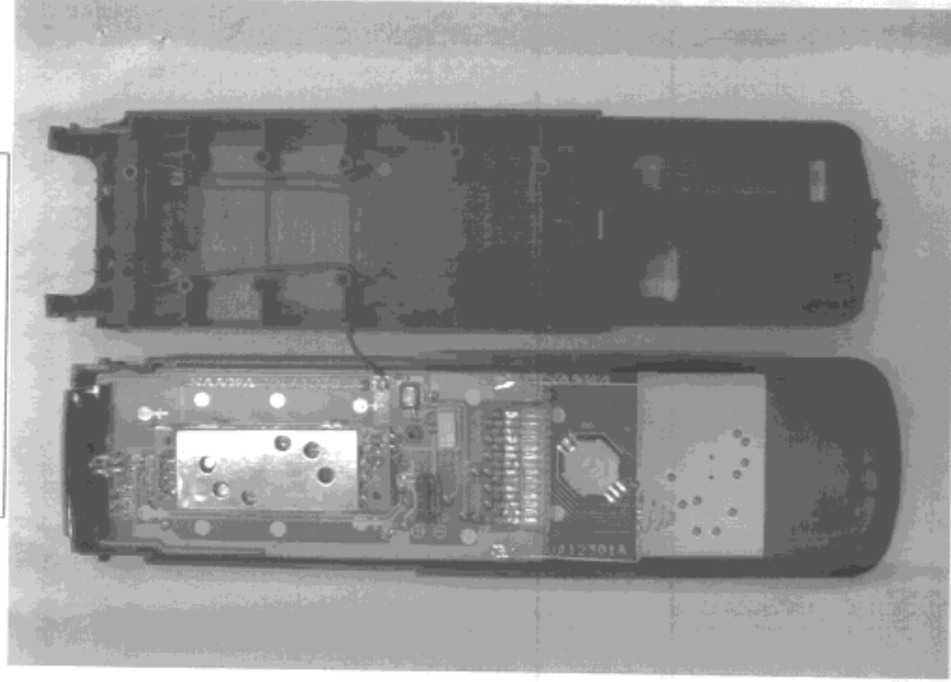
REAR VIEW: ENCLOSURE OPENED You will see a RF unit mounted on the main printed circuit board.
