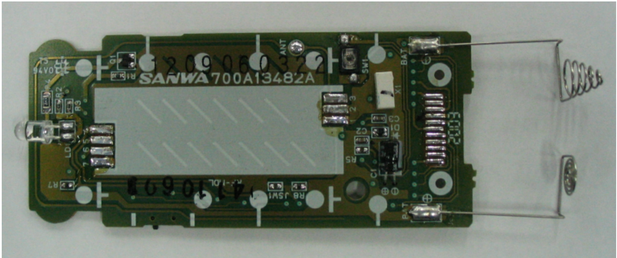
FCC ID:L73RM-Y822 MAIN PCB-A REAR VIEW
