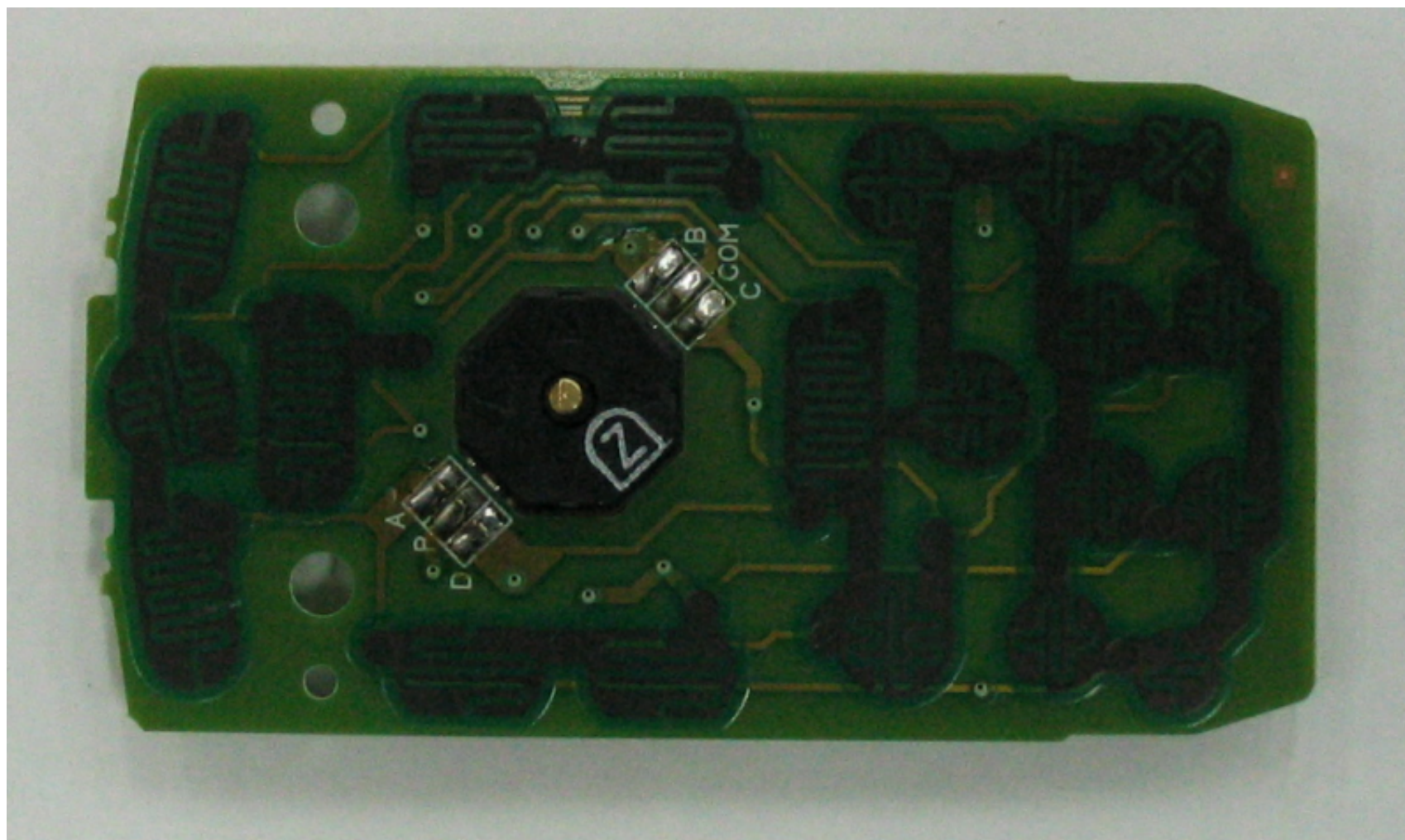
FCC ID:L73RM-Y822 MAIN PCB-B FRONT VIEW
