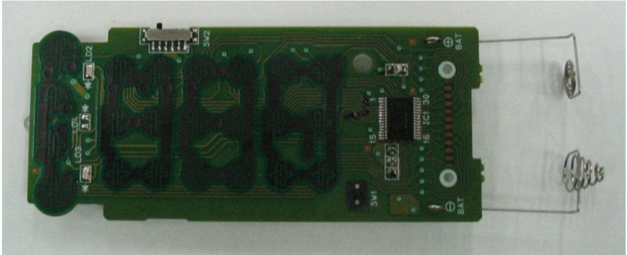
FCC ID:L73RM-Y822 MAIN PCB-A FRONT VIEW
