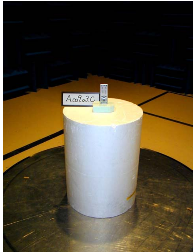
Vertically placed
