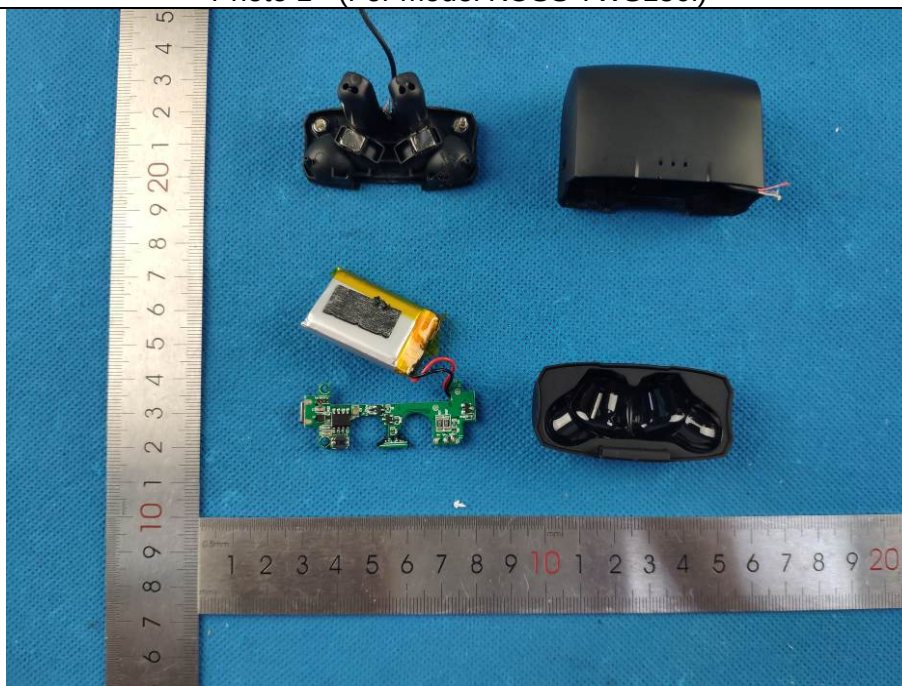
Photo 1 (For model KOSS TWS150i)
