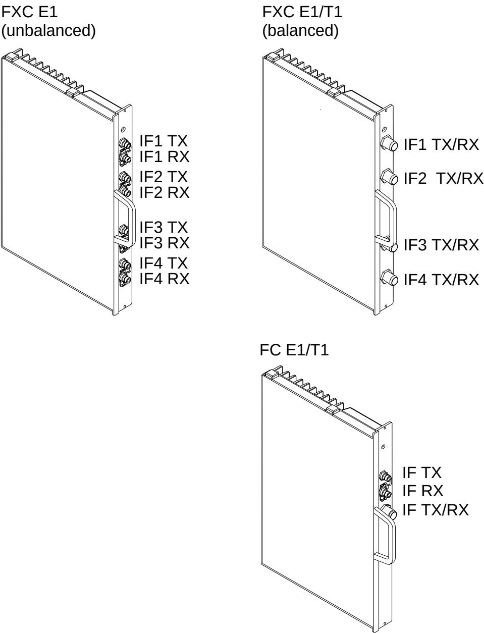
Figure 26. Wireline transmission unit alternatives
