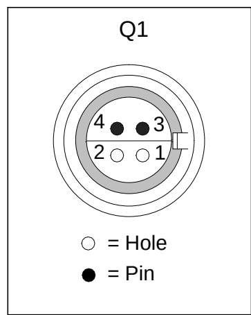
Figure 22. Pin order of Q1 connector
