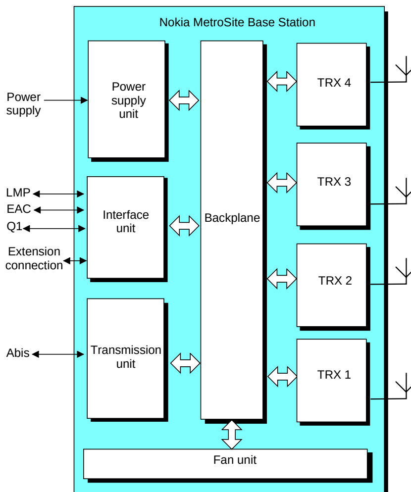
Figure 12. Nokia MetroSite BTS block diagram
