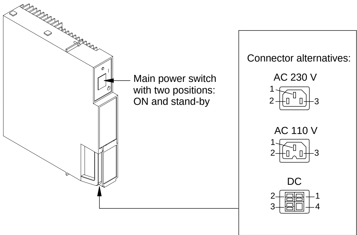
Figure 27. Power supply unit
